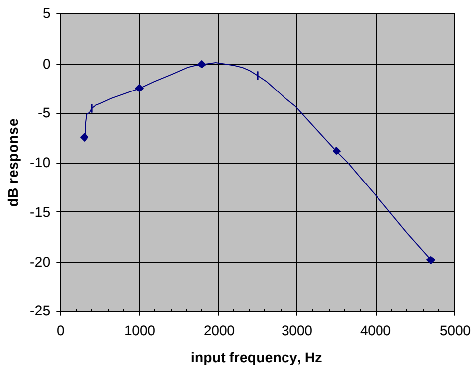
frequency response, 1 kHz deviation
