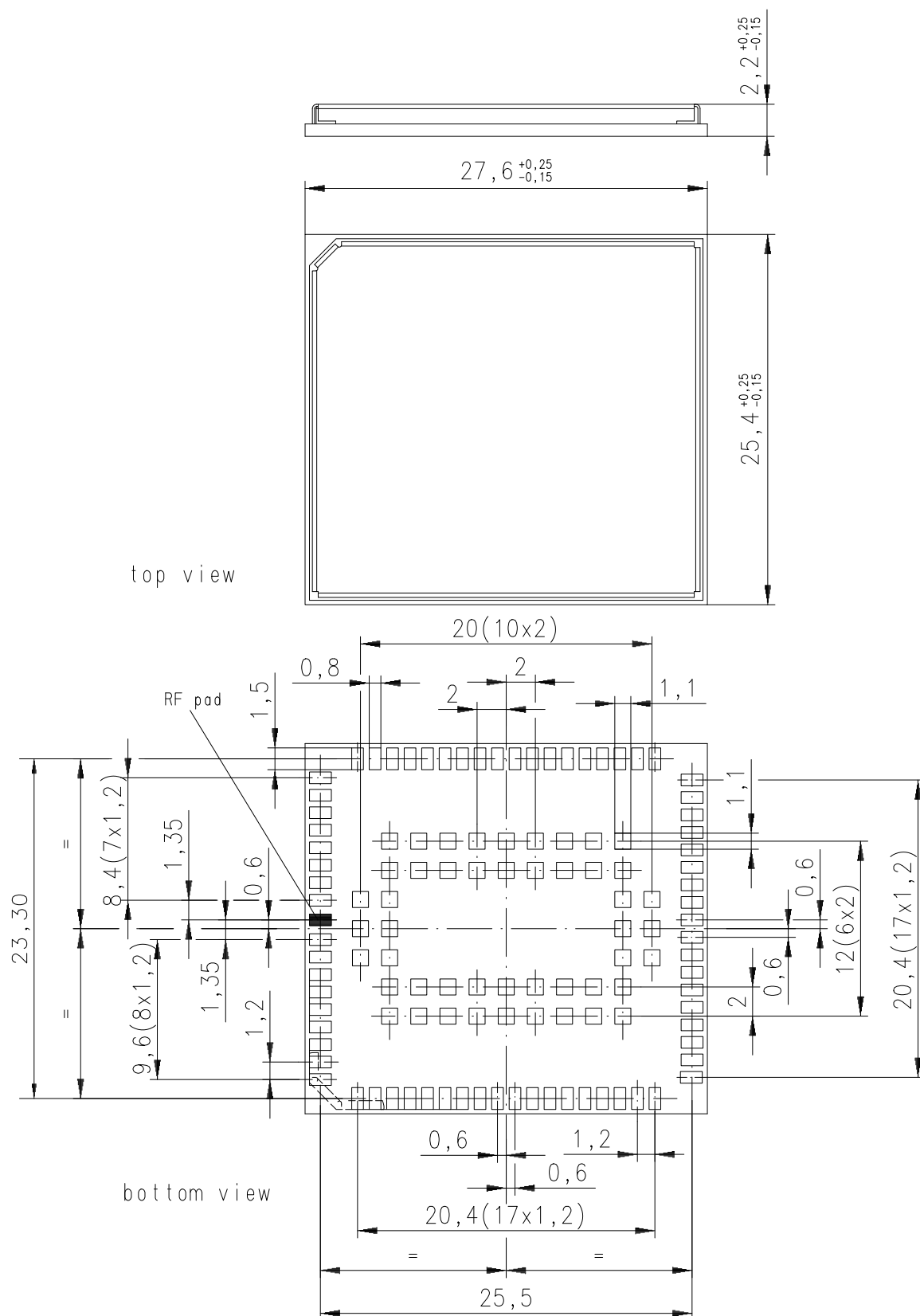
Figure 8: Dimensions of EHS6-A (all dimensions in mm)
