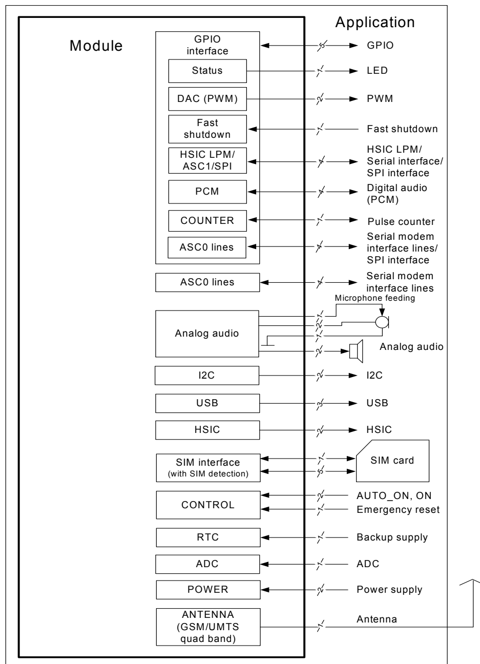
Figure 1: EHS6-A system overview
