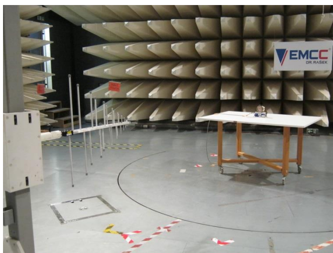
Radiated emissions measurement at 3 m distance, 250 MHz – 1000 MHz
