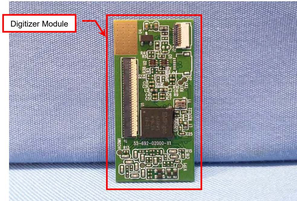
EUT Photo (90)
