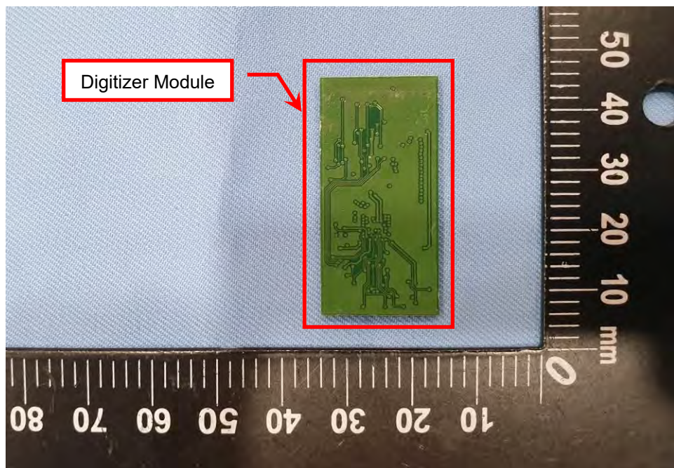
EUT Photo (90)
