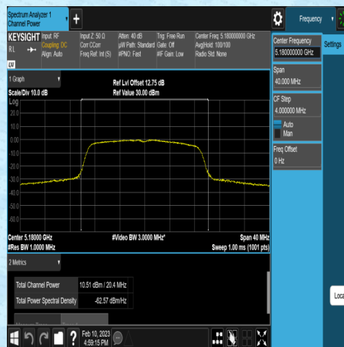
11AC20MIMO-Ant2-5180-NA----10.26-94.44-0.25
