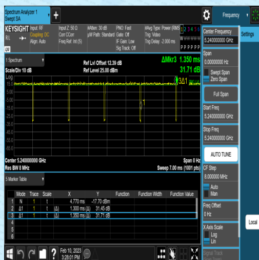
NTVN-11N20MIMO-Ant1-5240-1.30-1.35
