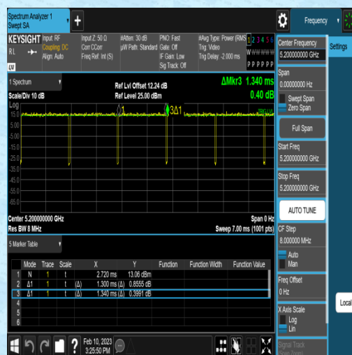
NTVN-11N20MIMO-Ant2-5200-1.30-1.34
