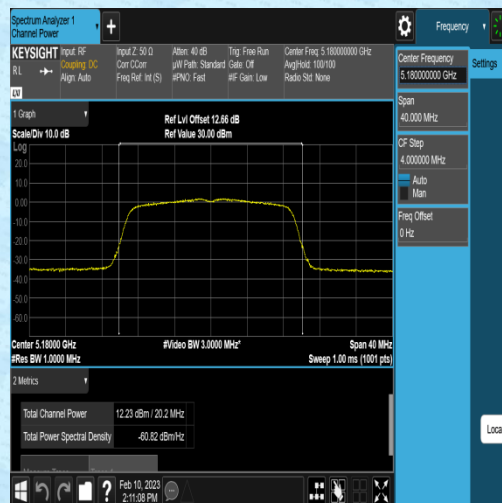
11AC20SISO-Ant2-5180-NA----12.07-96.32-0.16
