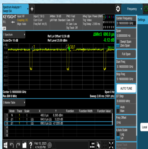
NTVN-11N40MIMO-Ant1-5190-0.64-0.69
