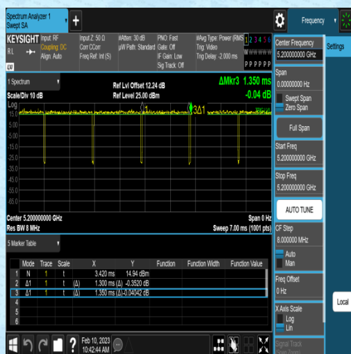
NTNV-11N20SISO-Ant2-5200-1.30-1.35
