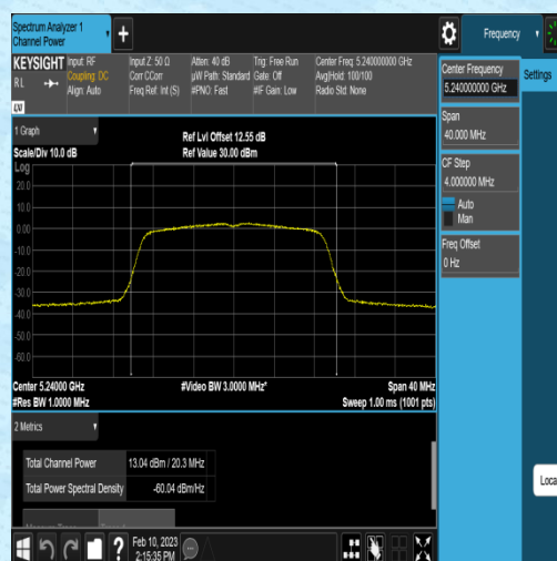
11AC20SISO-Ant2-5240-NA----12.88-96.32-0.16
