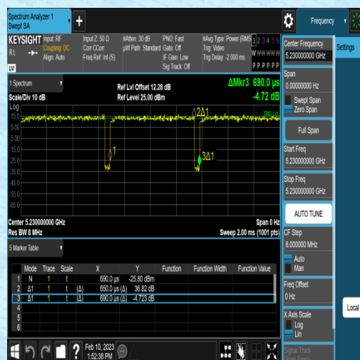
NTNV-11N40SISO-Ant2-5230-0.65-0.69
