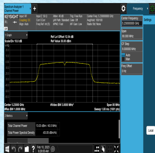
11AC40SISO-Ant1-5230-NA----12.77-94.20-0.26
