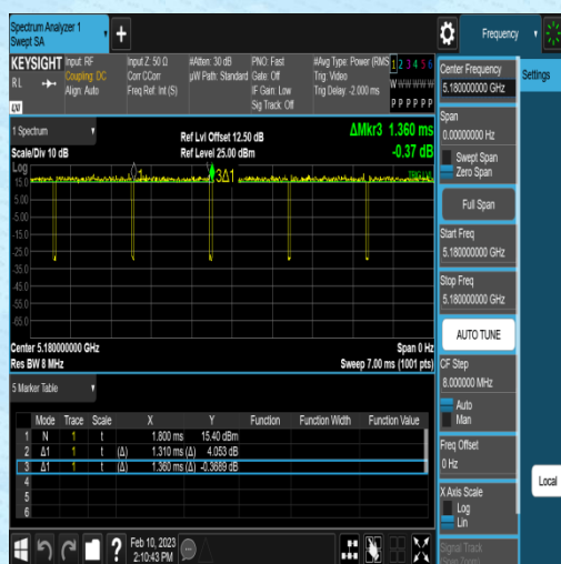
NTNV-11AC20SISO-Ant2-5180-1.31-1.36
