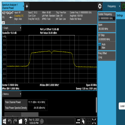
11AC40MIMO-Ant1-5190-NA----10.53-87.50-0.58
