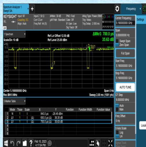
NTVN-11N40MIMO-Ant2-5190-0.65-0.70
