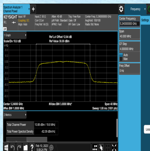
11AC20MIMO-Ant2-5240-NA----10.63-94.44-0.25
