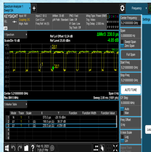
NTNV-11AC80MIMO-Ant2-5210-0.19-0.23
