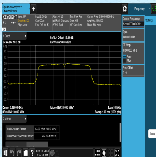
11AC40SISO-Ant1-5190-NA----12.95-92.86-0.32
