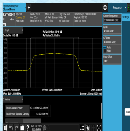
11AC20MIMO-Ant2-5200-NA----9.93-94.44-0.25
