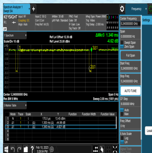
NTVN-11N20MIMO-Ant2-5240-1.30-1.34
