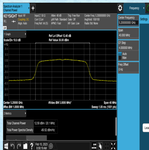
11AC20SISO-Ant1-5200-NA----12.34-96.32-0.16
