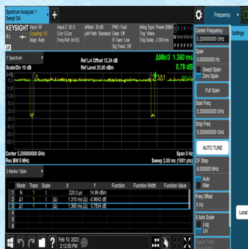
NTNV-11AC20SISO-Ant2-5200-1.31-1.36
