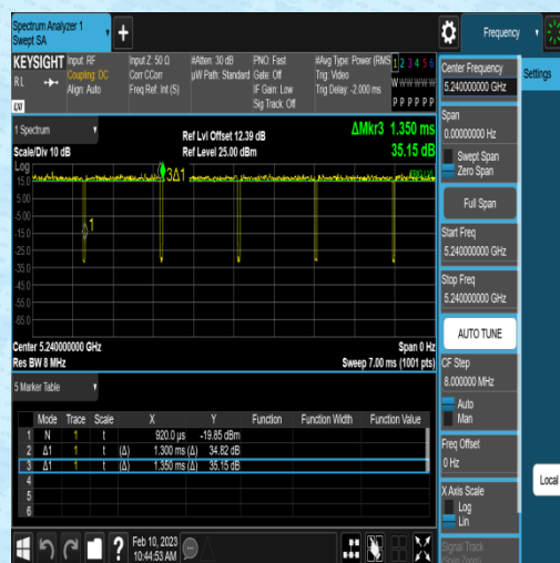
NTNV-11N20SISO-Ant2-5240-1.30-1.35
