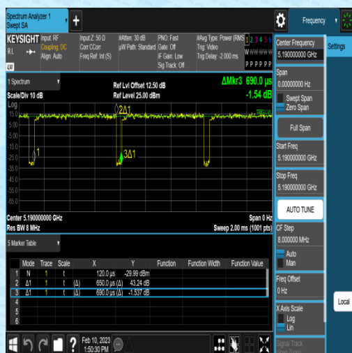
NTNV-11N40SISO-Ant2-5190-0.65-0.69
