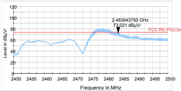
802.11g-Channel 11 Peak
