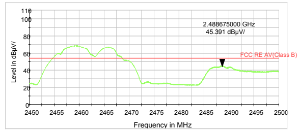
802.11b-Channel 11 Average
