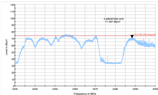
802.11ax HE40-Channel 9 Peak
