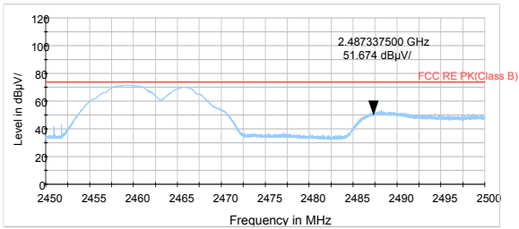
802.11b-Channel 11 Peak
