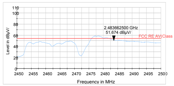
802.11g-Channel 11 Average
