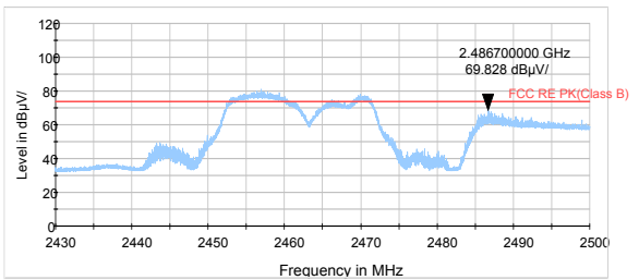
802.11ax HE20 -Channel 11 Peak
