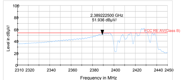
802.11n HT40 -Channel 3 Average
