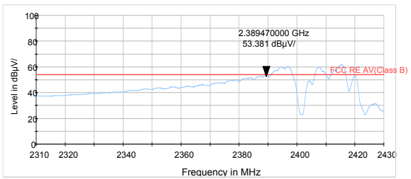
802.11g-Channel 1 Peak
