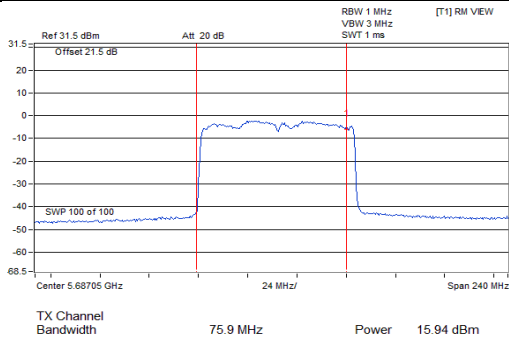
802.11ax (HE80)_Chain 1 / CH138 (U-NII-2C Band)
