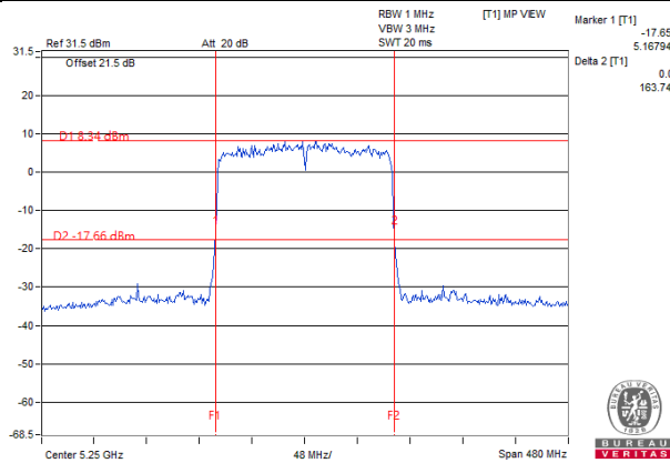
802.11ax (HE160)_Chain 0 / CH50 (U-NII-2A Band)
