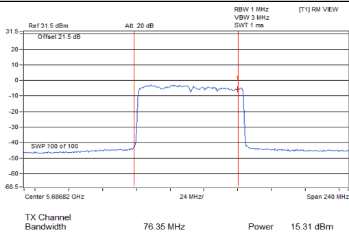
802.11ax (HE80)_Chain 0 / CH138 (U-NII-2C Band)
