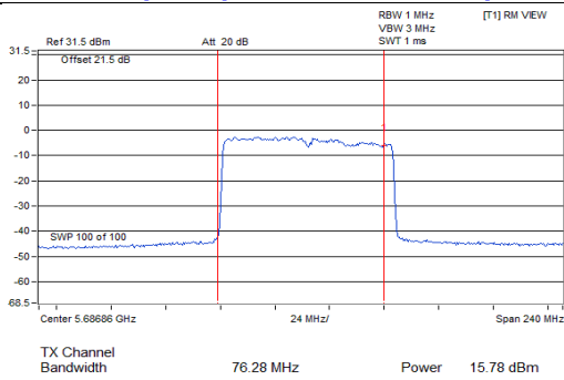
802.11ax (HE80)_Chain 3 / CH138 (U-NII-2C Band)
