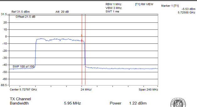
802.11ax (HE80)_Chain 0 / CH138 (U-NII-3 Band)
