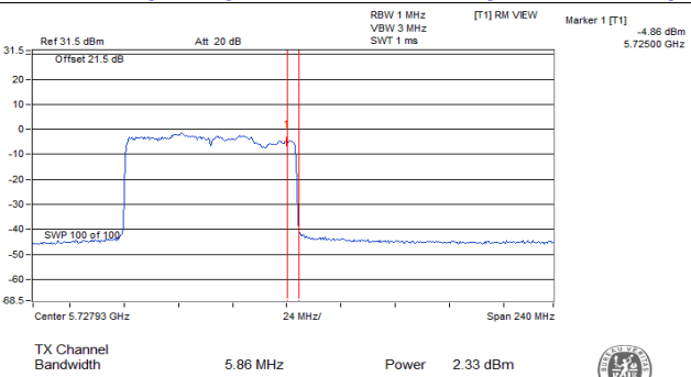
802.11ax (HE80)_Chain 3 / CH138 (U-NII-3 Band)
