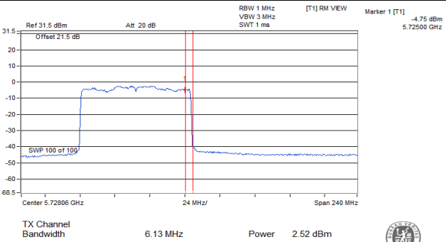
802.11ax (HE80)_Chain 1 / CH138 (U-NII-3 Band)
