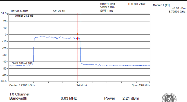
802.11ax (HE80)_Chain 2 / CH138 (U-NII-3 Band)
