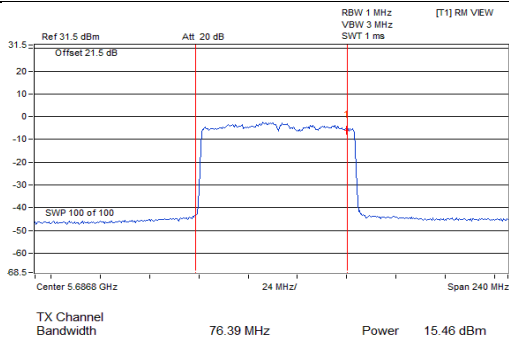
802.11ax (HE80)_Chain 2 / CH138 (U-NII-2C Band)
