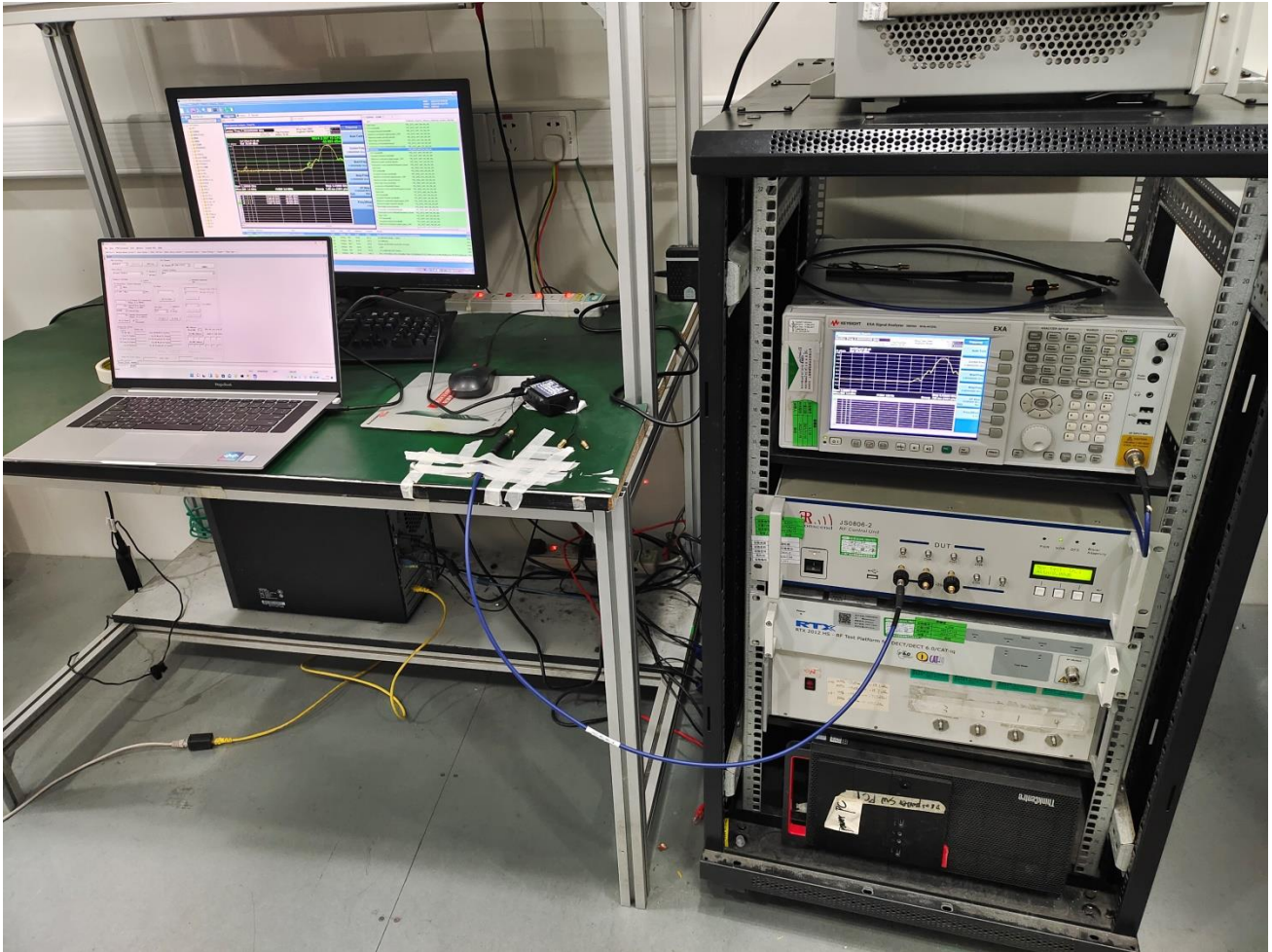
BT/BLE/2.4G WiFi/5G WiFi Test setup
