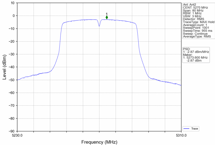
802.11ac(VHT40)_LCH_5270MHz_MIMO_NTNV
