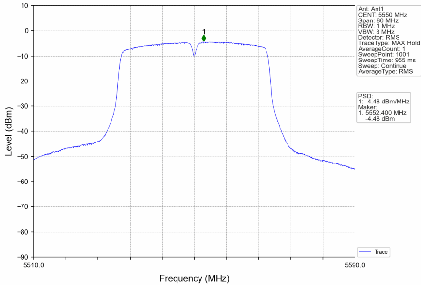
802.11ac(VHT40)_MCH_5550MHz_Ant1_NTNV
