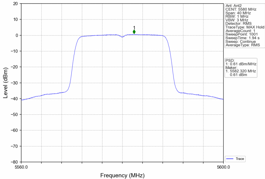
802.11ac(VHT20)_MCH_5580MHz_MIMO_NTNV
