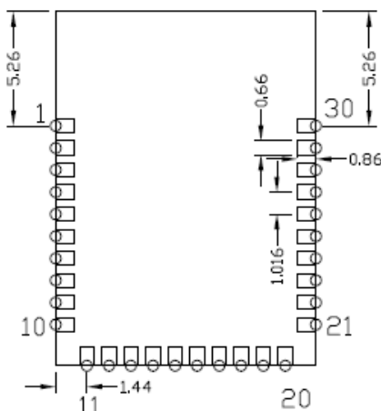
Figure 3. Solder Pad Dimensions (Seen from Bottom)
