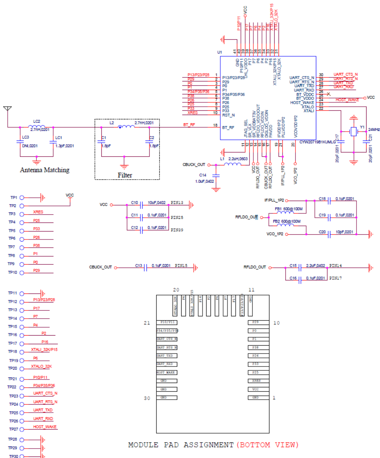
Figure 9. CYBT-413034-02 Schematic Diagram
