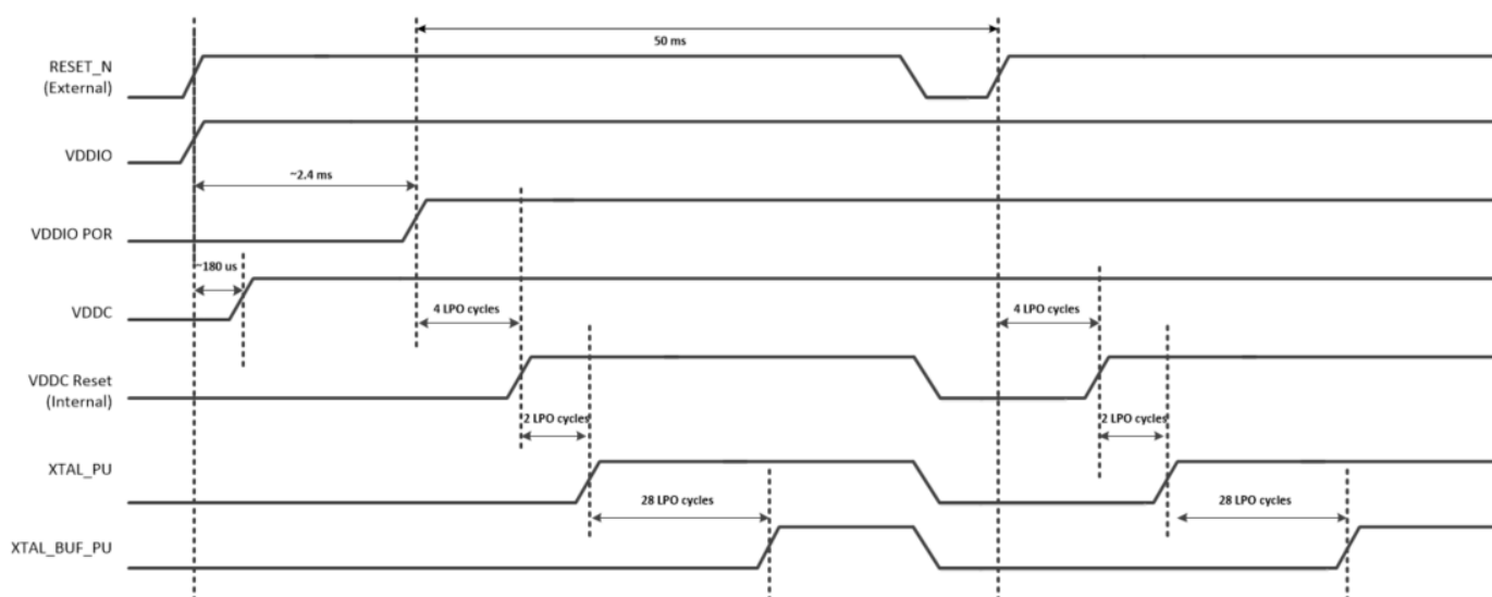
Figure 11. Reset Timing
