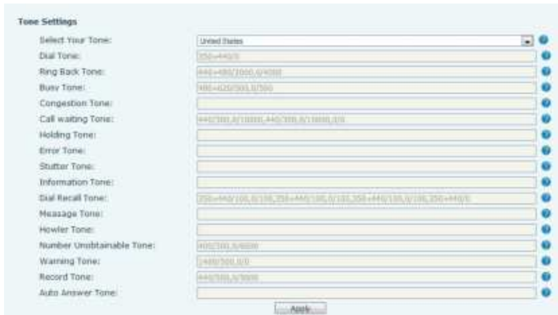
Picture 132 - Tone settings on the web
