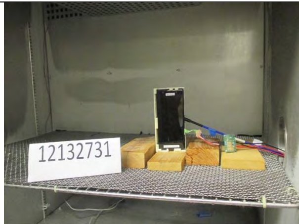
FREQUENCY STABILITY
