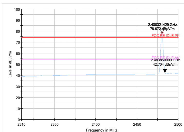
Fig 49 Radiated emission (Power): \pi/4 DQPSK, high channel
