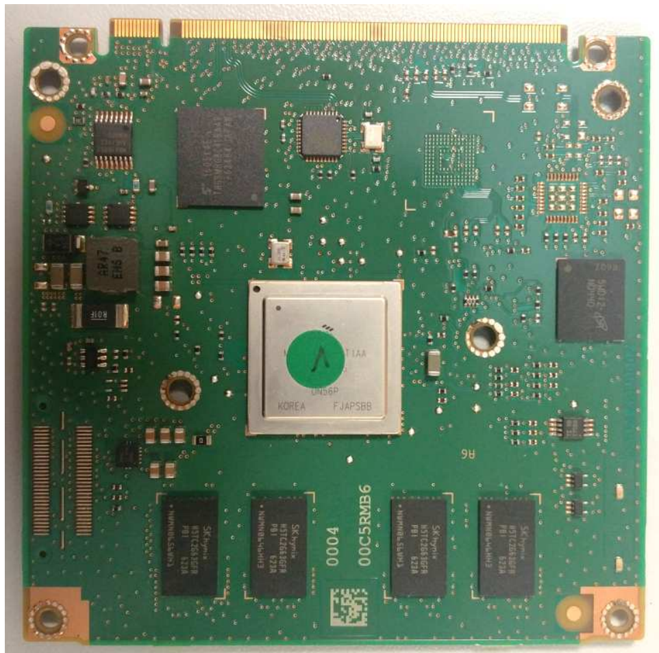
Daughterboard Top
