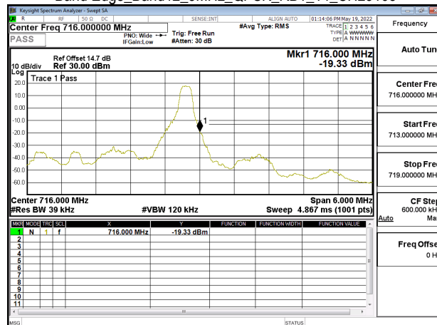
Band Edge_Band12_3MHz_QPSK_RB15_0_CH23025
