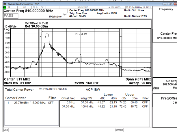
Emission Mask_Band26-Part90s_5MHz_QPSK_RB1_0_CH26740
