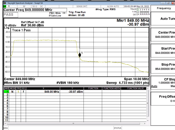
Band Edge_Band5_5MHz_QPSK_RB25_0_CH20625
