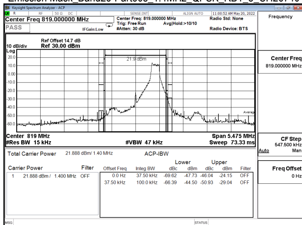
Emission Mask_Band26-Part90s_1.4MHz_QPSK_RB1_5_CH26740
