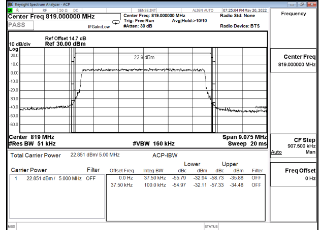
Emission Mask_Band26-Part90s_5MHz_QPSK_RB25_0_CH26740
