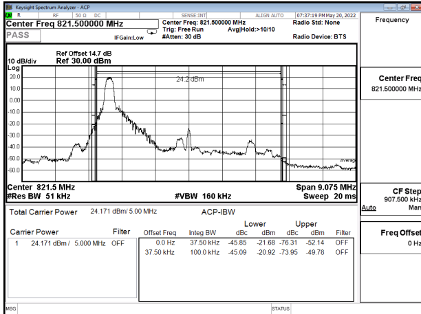
Emission Mask_Band26-Part90s_5MHz_QPSK_RB1_24_CH26715
