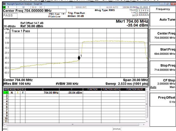
Band Edge_Band17_10MHz_QPSK_RB50_0_CH23780
