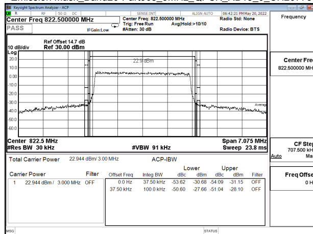
Emission Mask_Band26-Part90s_5MHz_QPSK_RB1_0_CH26715
