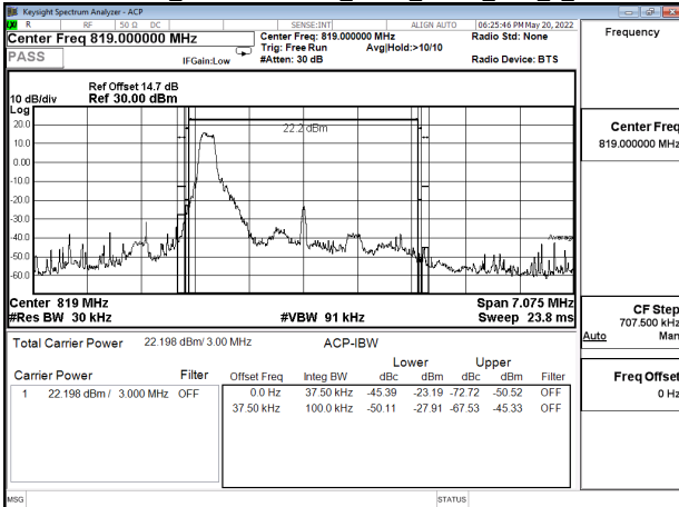
Emission Mask_Band26-Part90s_3MHz_QPSK_RB1_0_CH26740
