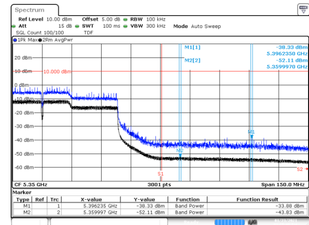
BE-R-HIGH, SISO-A, 802.11ac160-VHT0, Ch50
