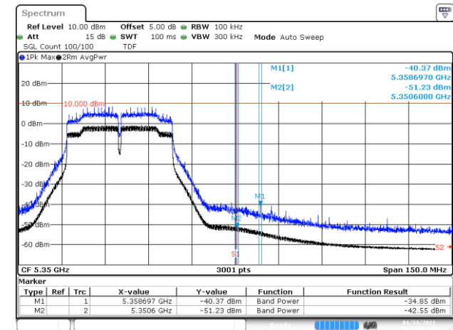
BE-R-HIGH, SISO-A, 802.11n40-HT0, Ch62
