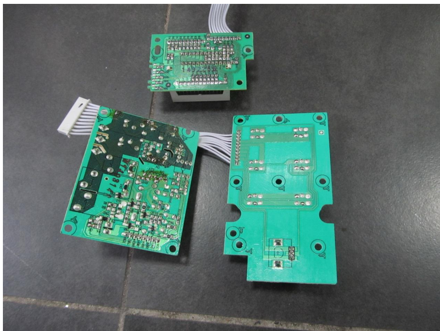
Mother board(Power board+LED display board+ Electronic Keyboard board) - Bottom View
