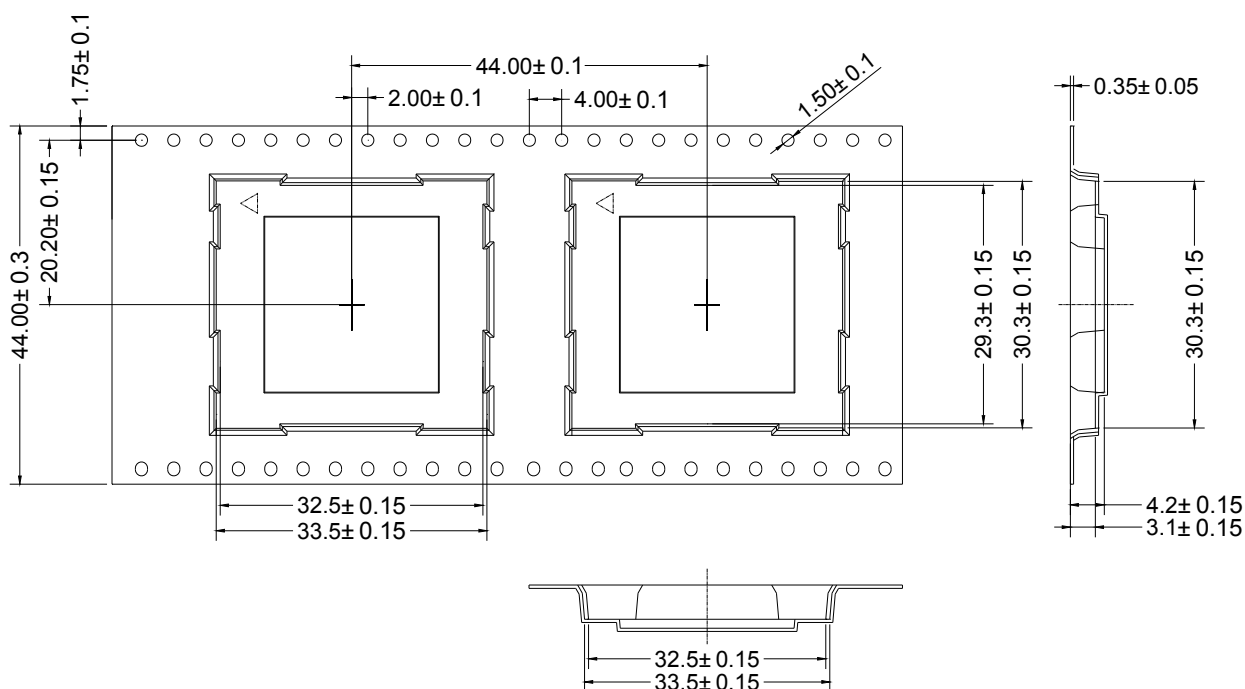
Figure 50: Tape Specifications
