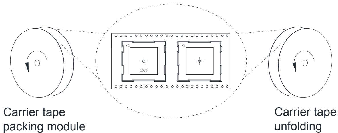
Figure 52: Tape and Reel Directions
