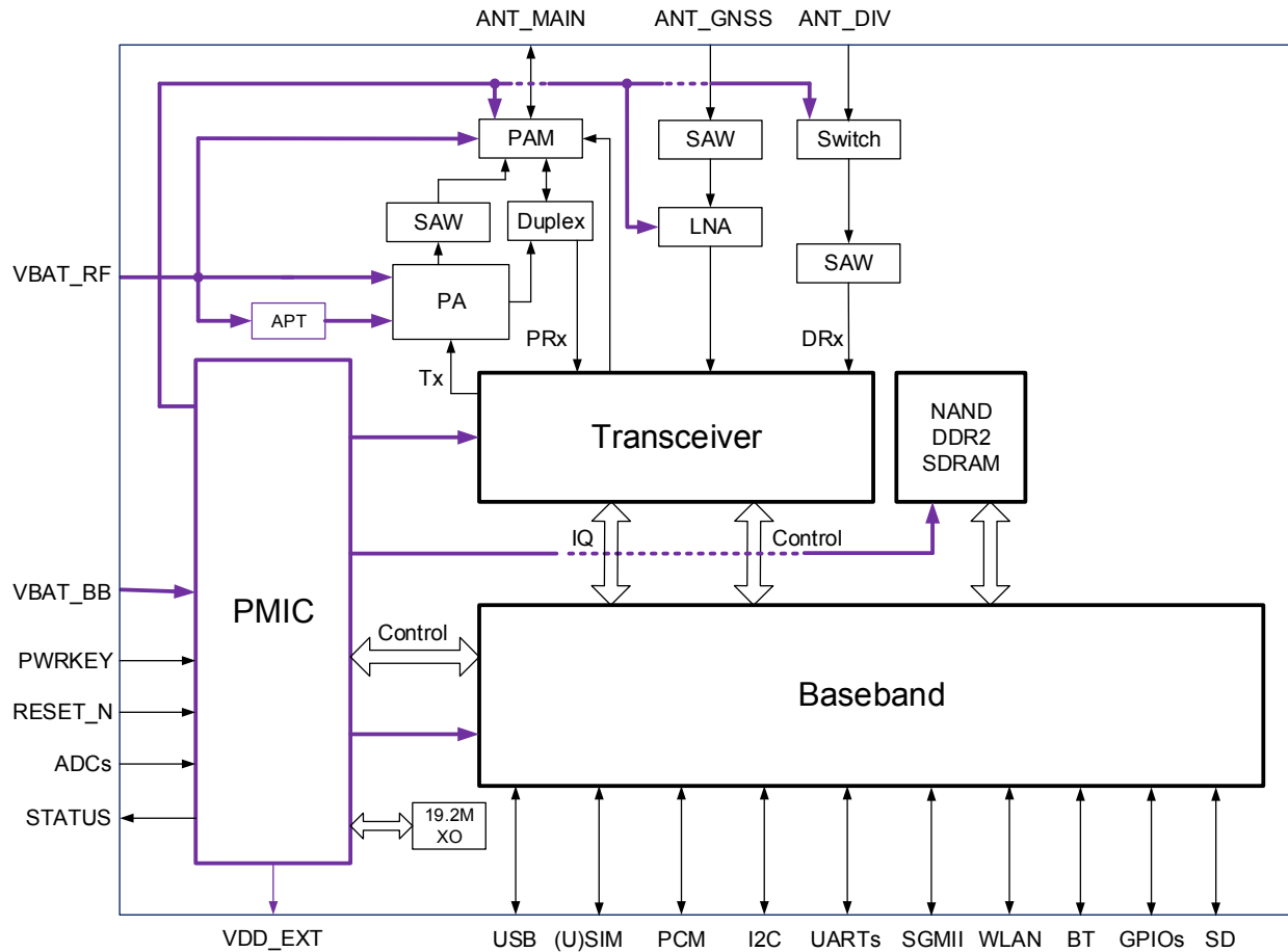
Figure 1: Functional Diagram
