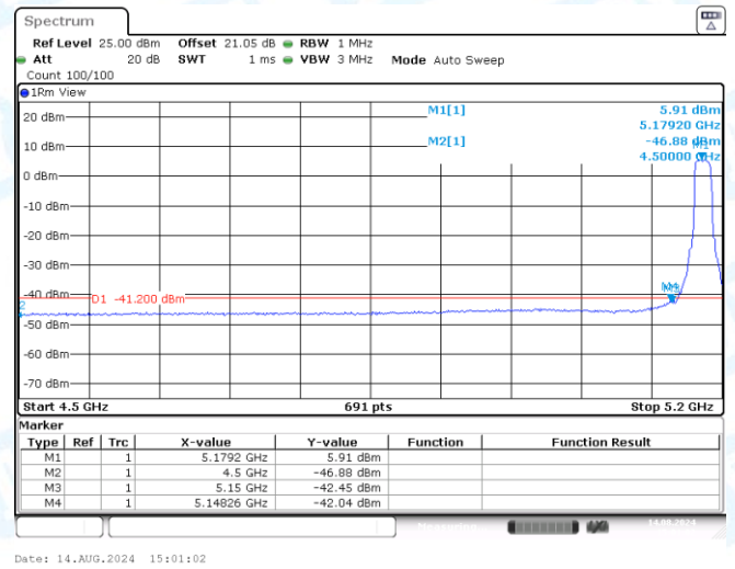
11A-Ant2-5180-PASS
