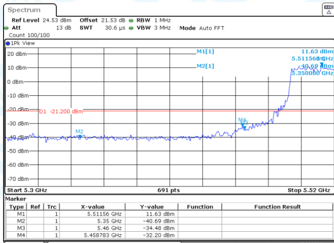
11AX40SISO-Ant2-5310-PASS
