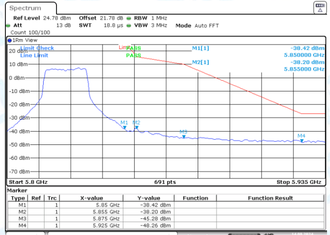
11N20SISO-Ant2-5825-PASS
