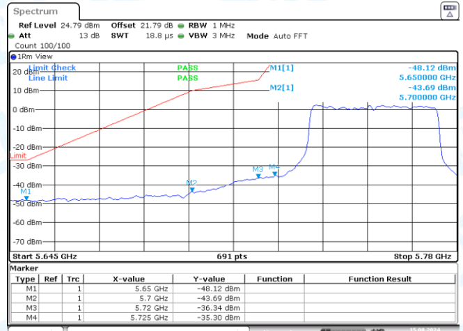
11AX40SISO-Ant2-5755-PASS
