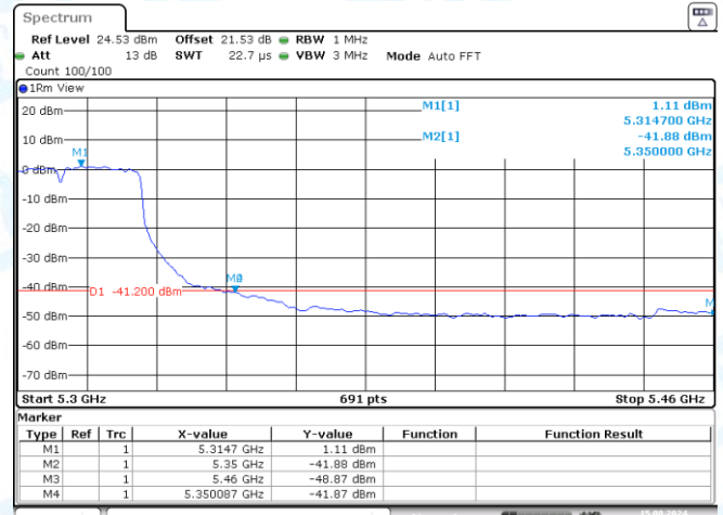
11AC40SISO-Ant2-5310-PASS
