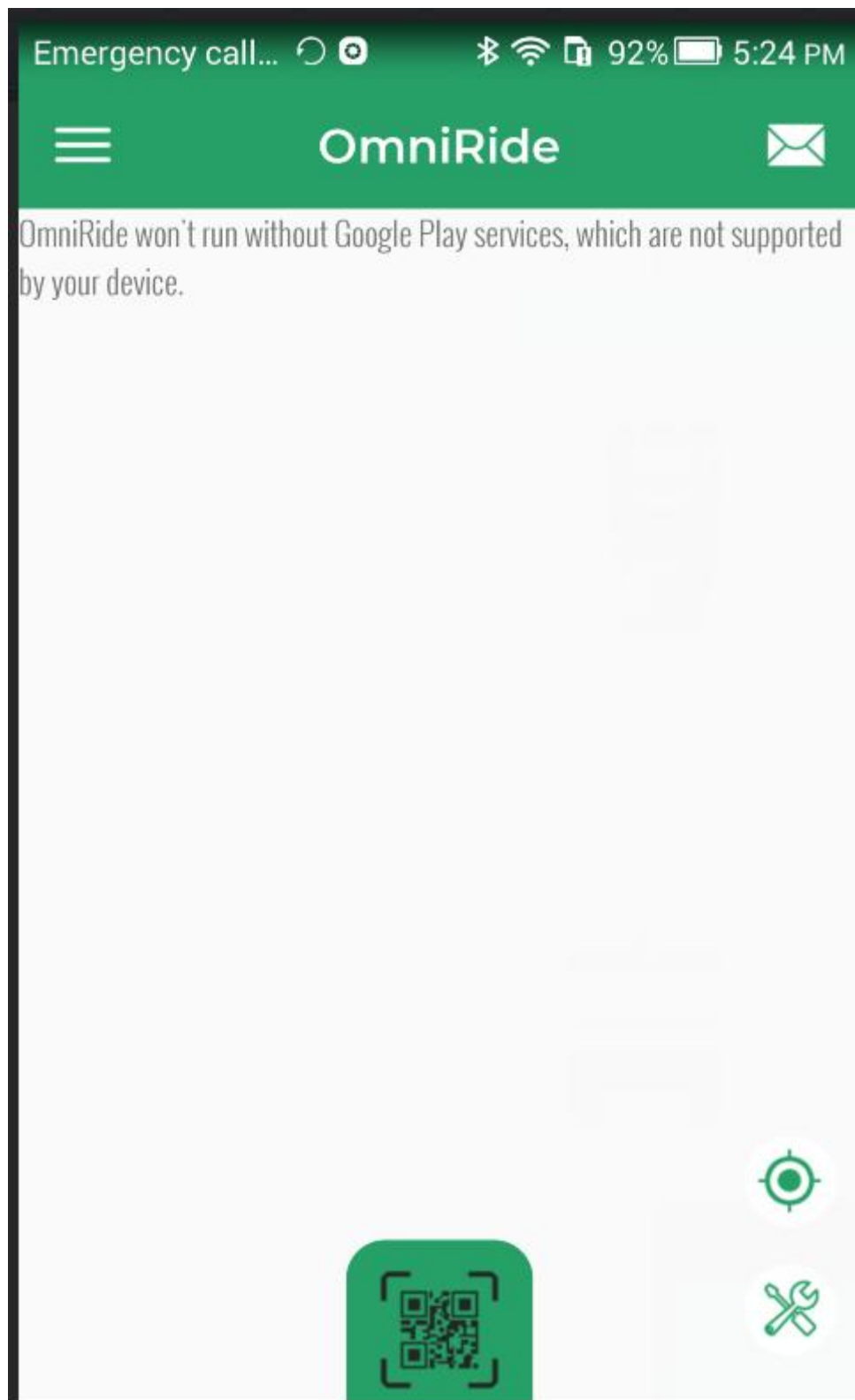
main page
