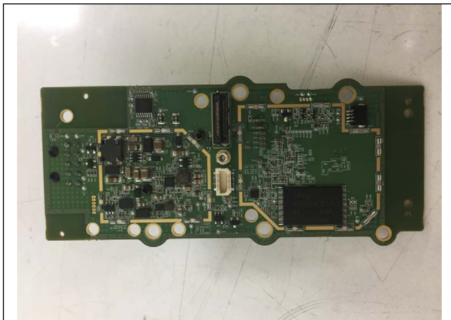
Bottom view of Sub1 PCB
