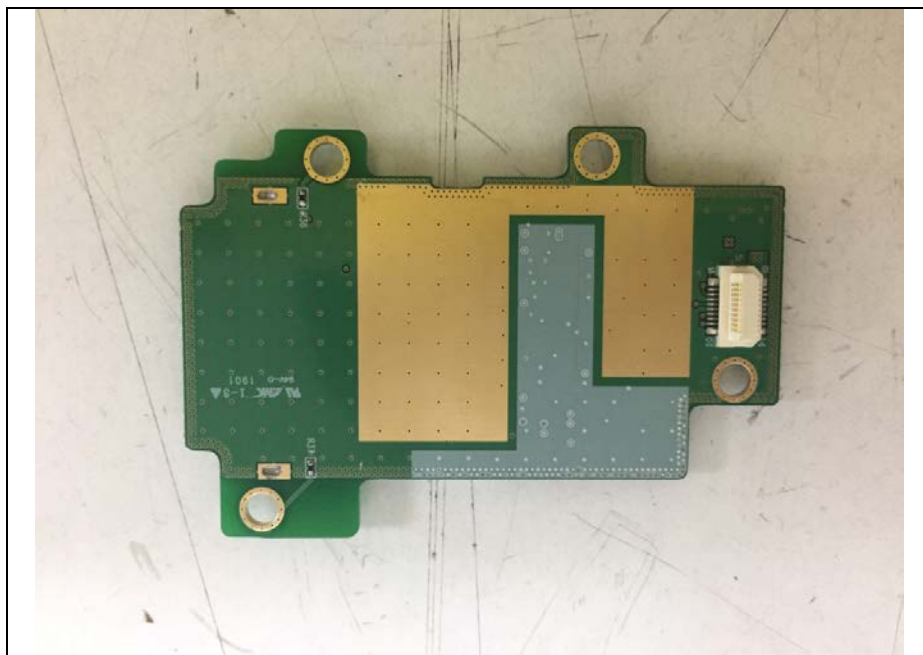
Bottom view of Sub3 PCB
