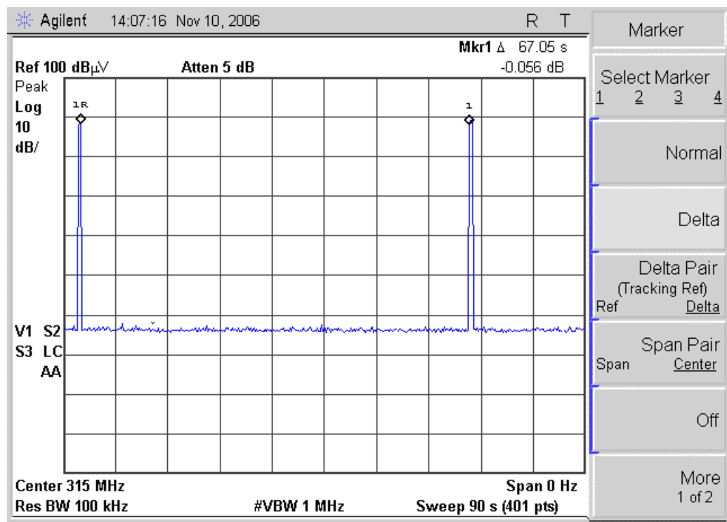
Figure 4. Transmission interval
