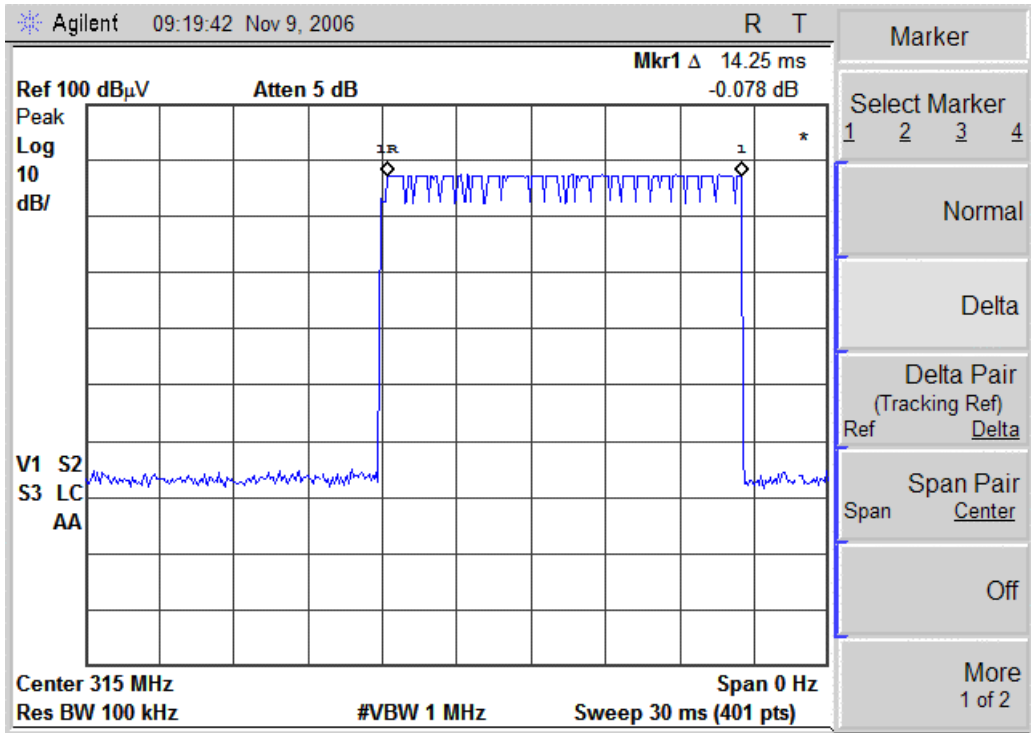
Figure 1. normal transmission
