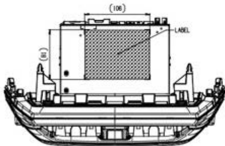
112 TOP VIEW
