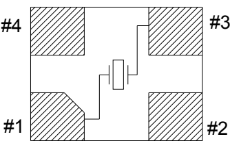
PIN CONNECTION (TOP VIEW)
