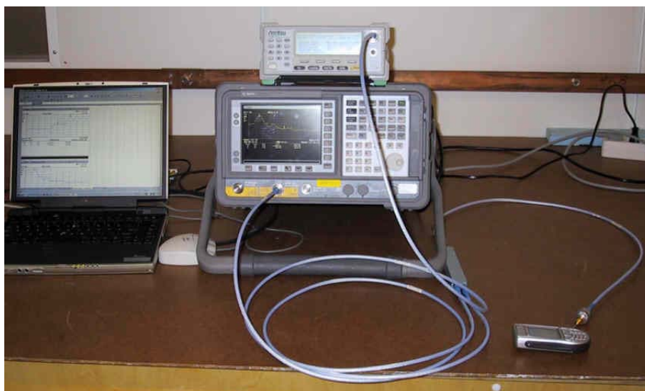
Picture 1: test set-up for conducted measurements from antenna port
