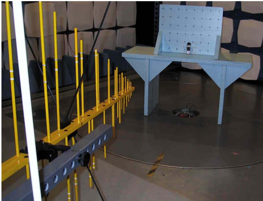
Picture 3: Radiated spurious emission measurement set-up for below 3 GHz measurements, EUT in vertical (V) orientation
