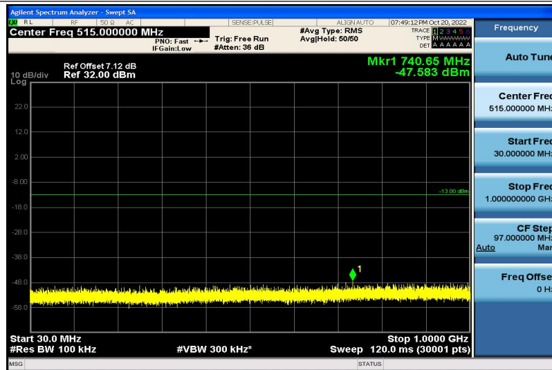
Band4-10MHz-16QAM-20000-1RB#0-30~1000MHz
