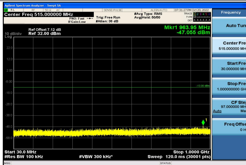
Band4-5MHz-16QAM-20175-1RB#0-30~1000MHz
