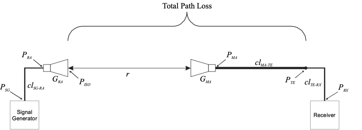
FIGURE 4-2 TYPICAL CONFIGURATION FOR MEASURING PATH LOSS
