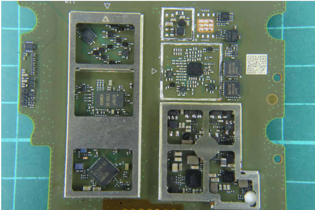
(35) EUT Photo (WWAN Module)
