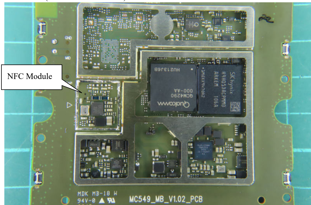
(34) EUT Photo (WLAN & BT Module)
