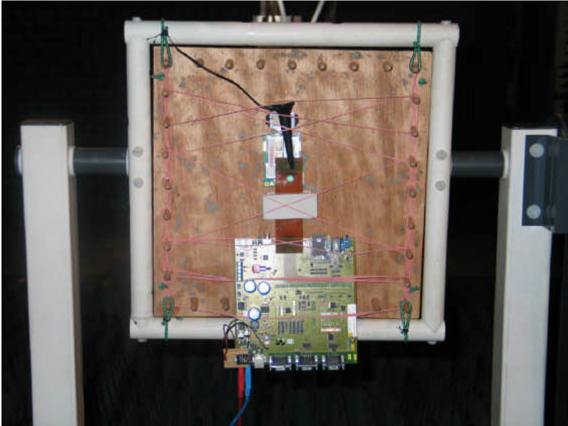
Photo 1: Test setup for radiated measurements
