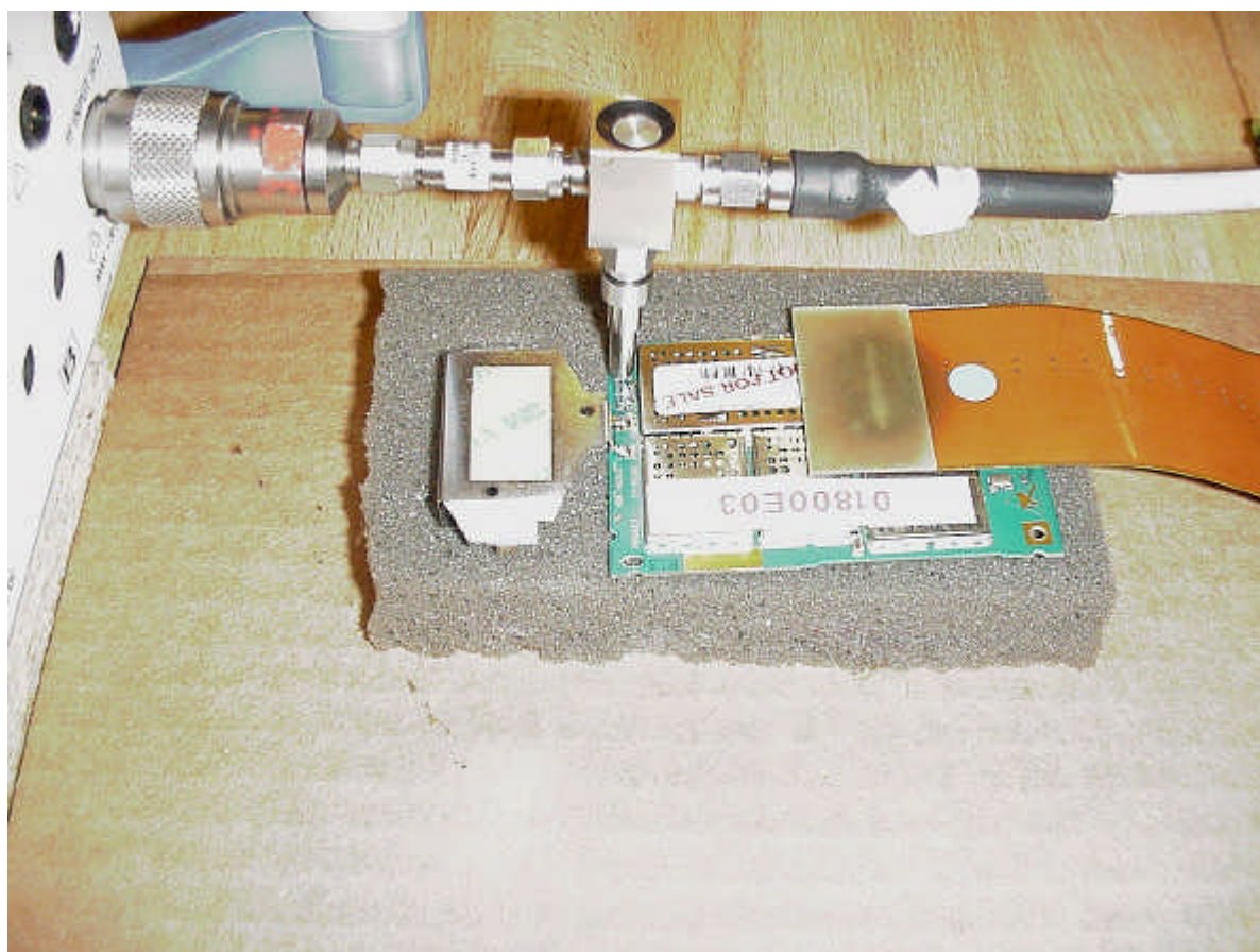
Photo 2: Test setup for conducted measurements
