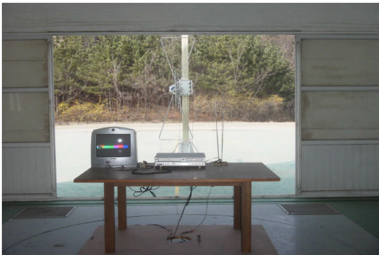
Front View
