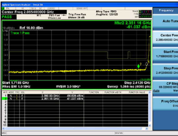
Antenna C
