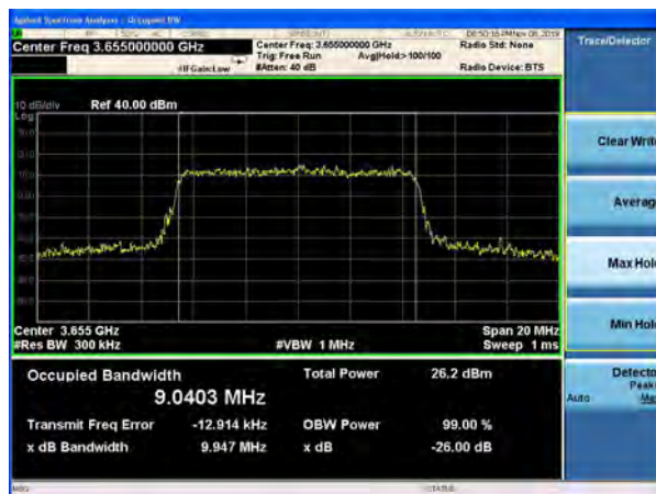
LTE Band 48 64QAM 10MHz CH-Middle
