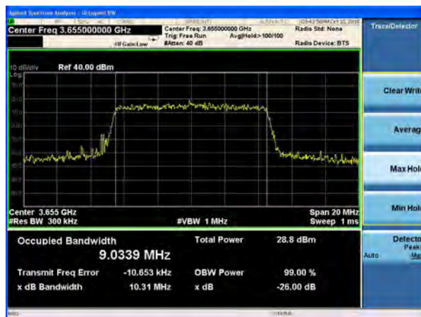
LTE Band 48 16QAM 10MHz CH-Middle
