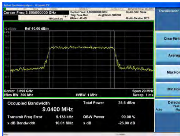
LTE Band 48 64QAM 10MHz CH-High
