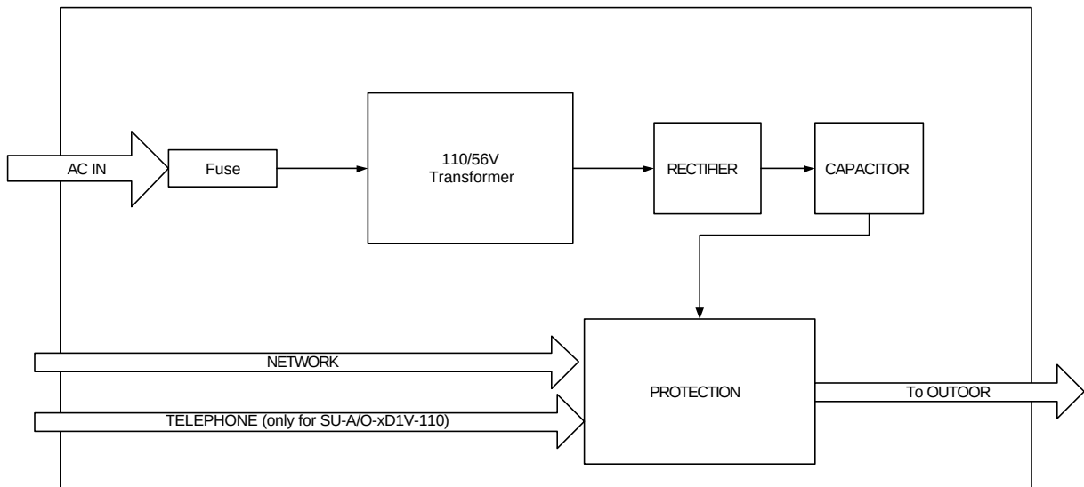
Fig 5. Indoor Unit
