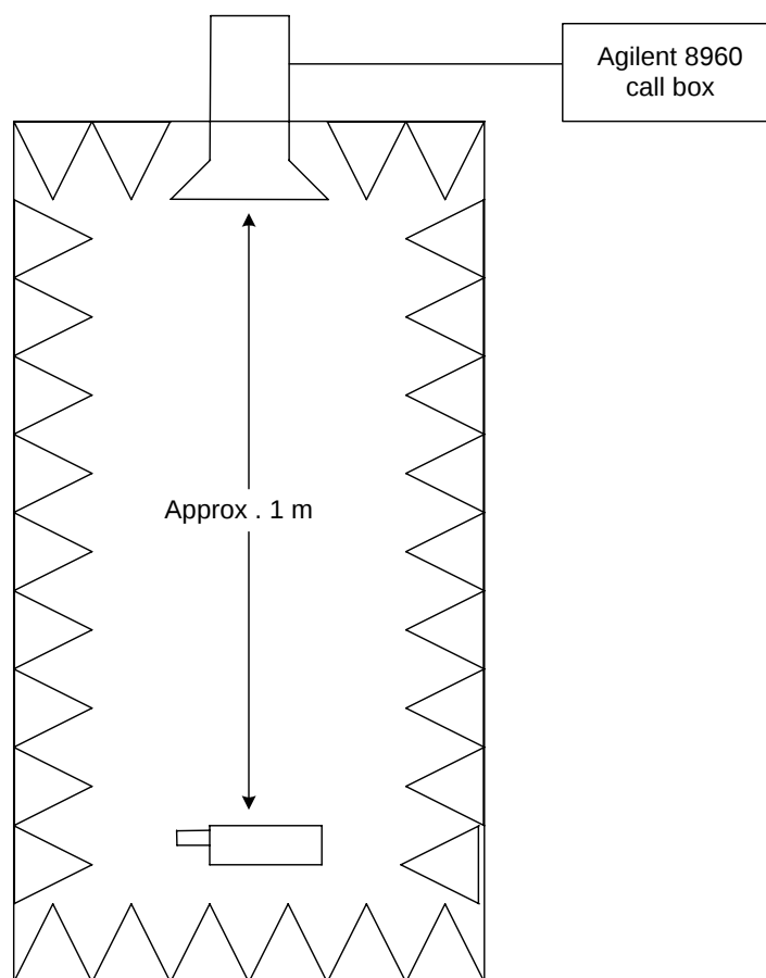
Figure 1: Anechoic chamber
