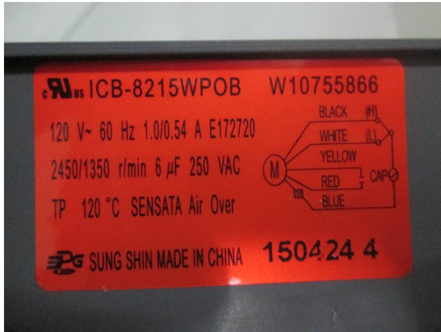
EUT – Exhaust Fans Label View
