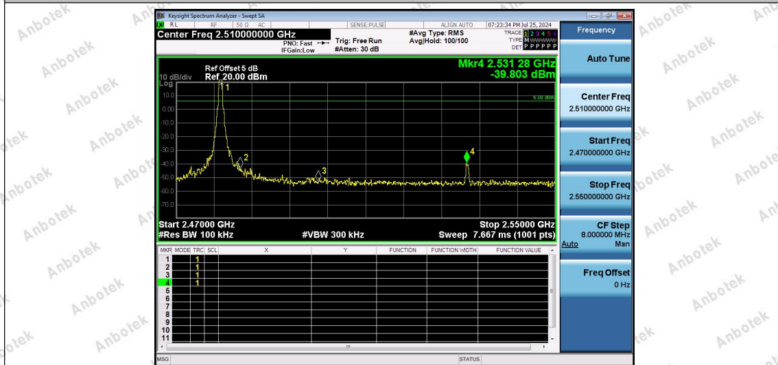
2.4G-Ant1-2479.4-PASS
