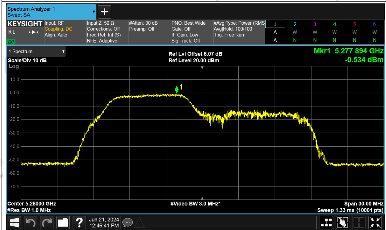
PSD NVNT be20 52+26RU Index 38+1 5280MHz Ant2
