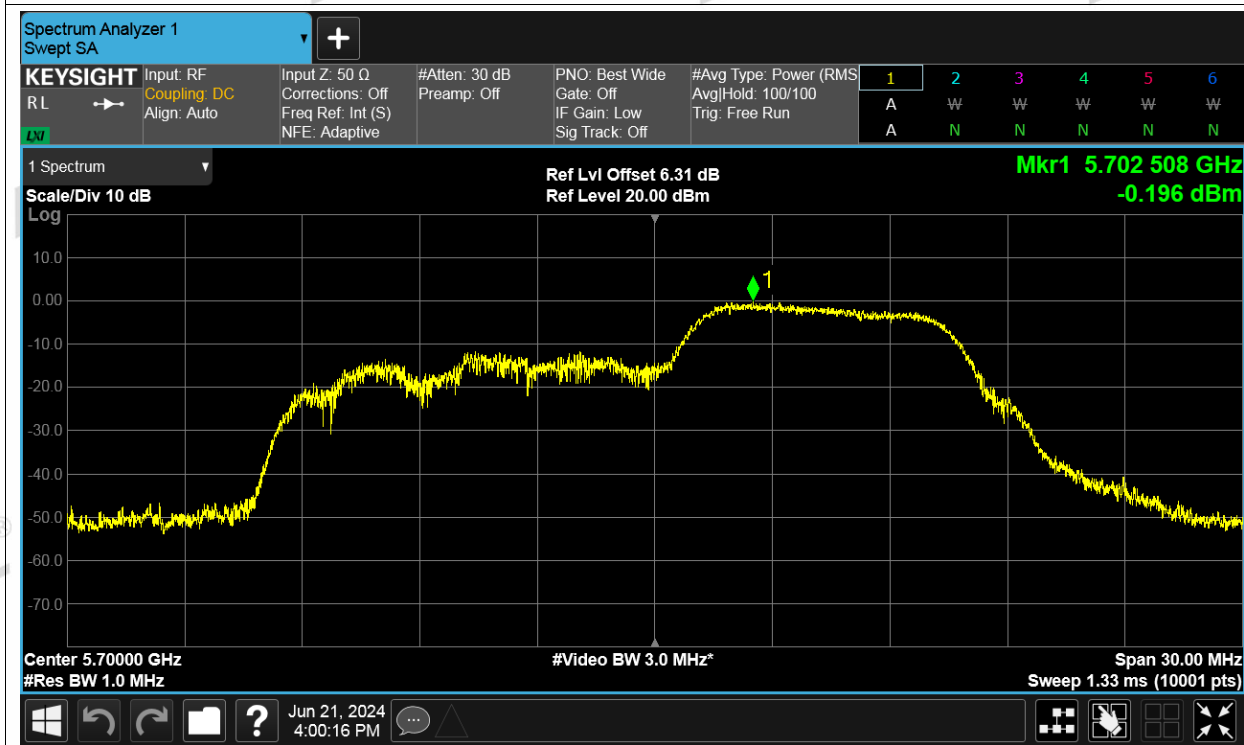
PSD NVNT be20 52+26RU Index 39+7 5700MHz Ant2
