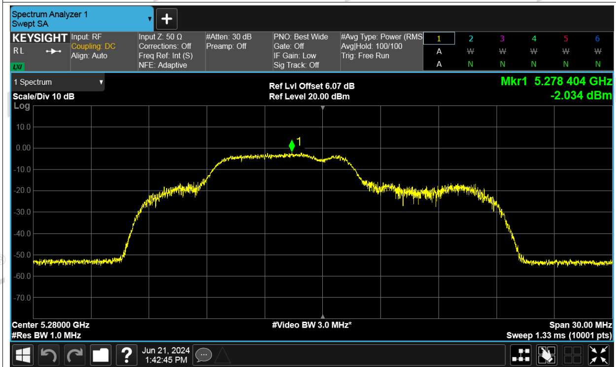
PSD NVNT be20 52+26RU Index 38+4 5280MHz Ant2
