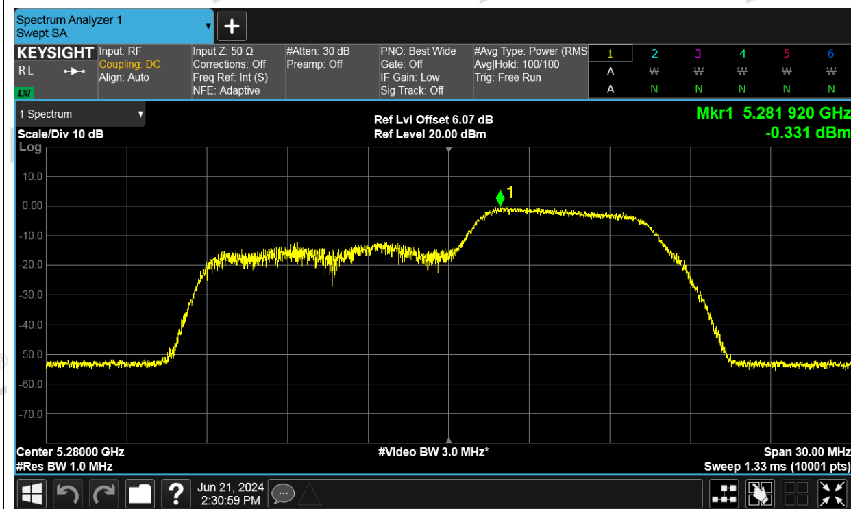
PSD NVNT be20 52+26RU Index 39+7 5280MHz Ant2
