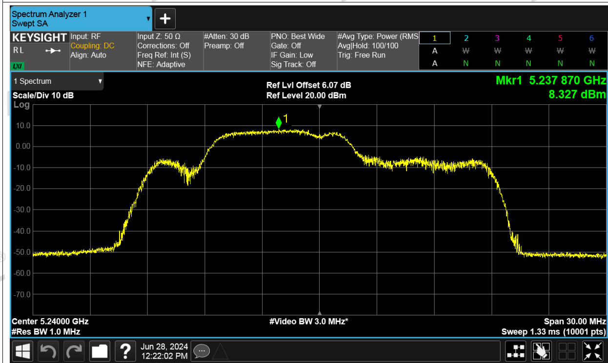
PSD NVNT be20 52+26RU Index 38+4 5240MHz Ant2
