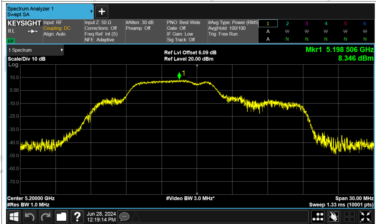
PSD NVNT be20 52+26RU Index 38+4 5200MHz Ant3
