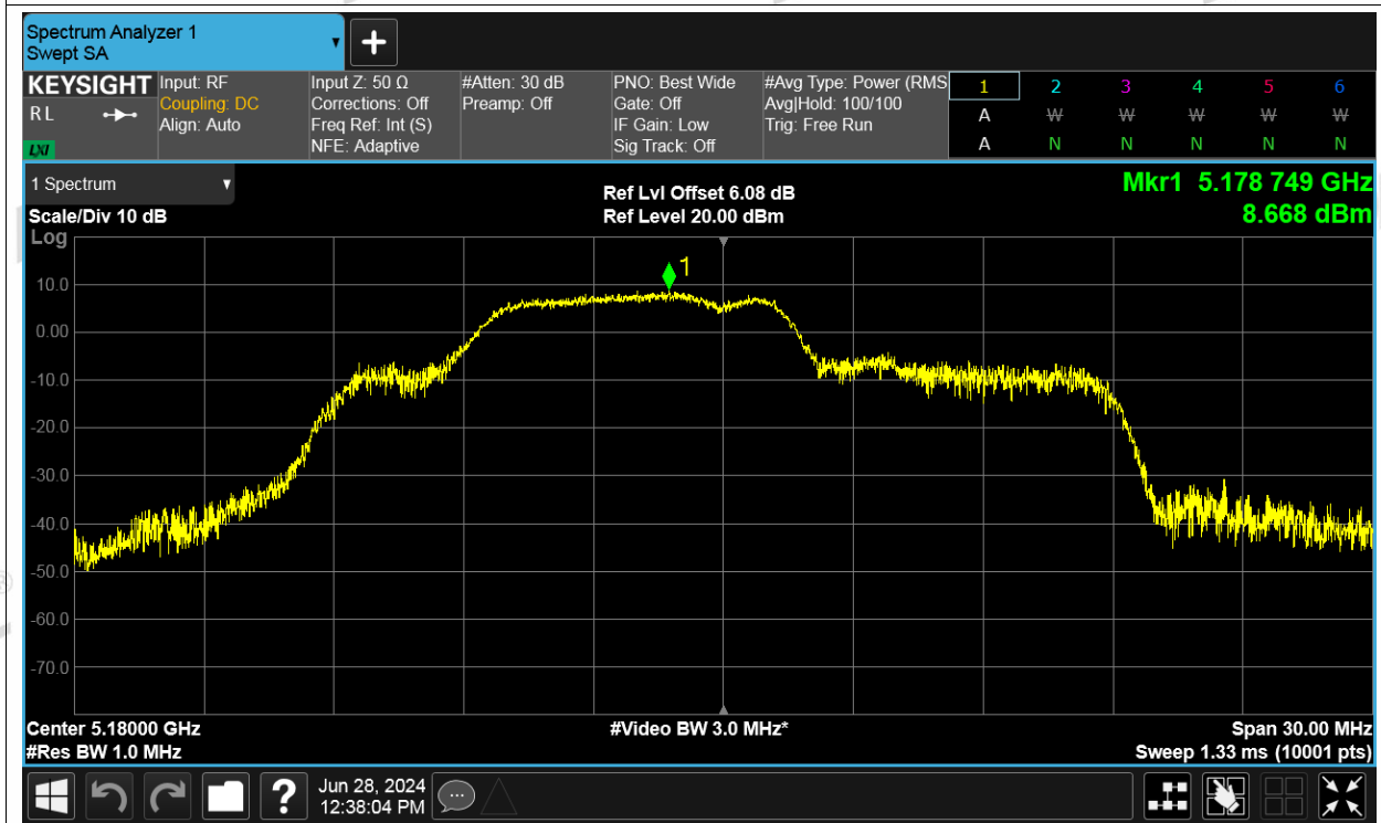
PSD NVNT be20 52+26RU Index 38+4 5180MHz Ant2
