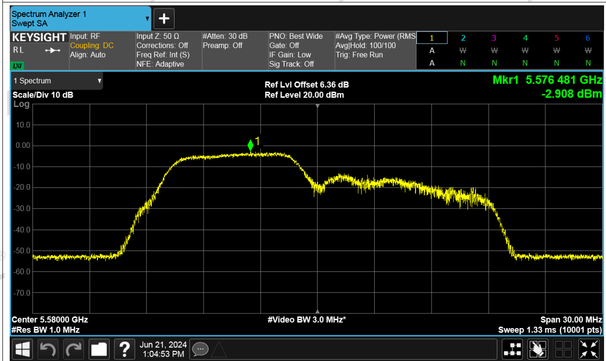
PSD NVNT be20 52+26RU Index 38+1 5580MHz Ant3
