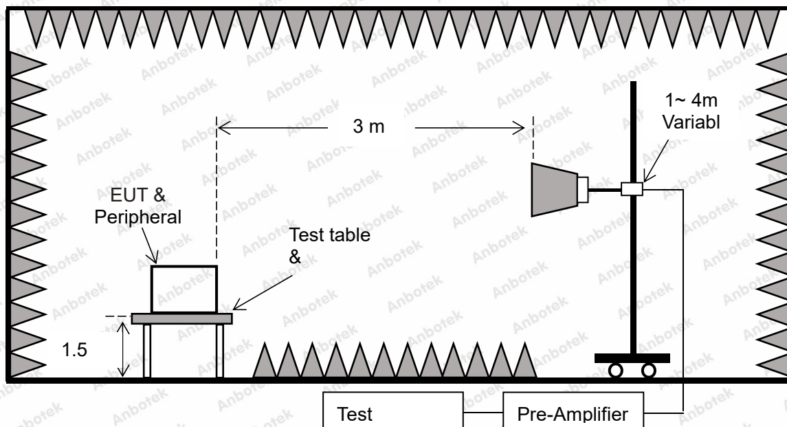
Figure 3. Above 1 GHz
