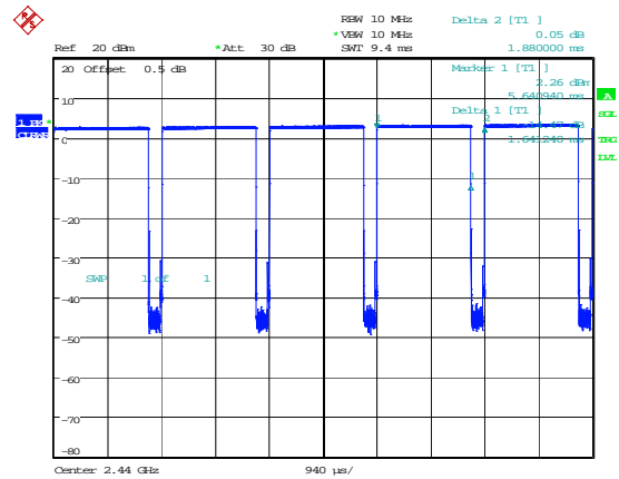
BLE_1M_Middle_Channel
