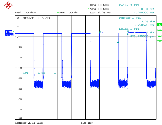
BLE_2M_Middle_Channel
