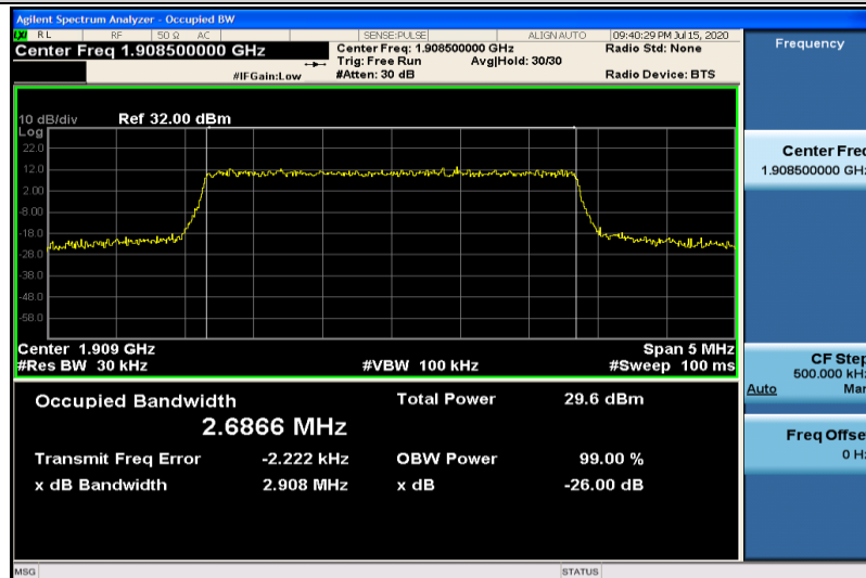
Band2-3MHz-16QAM-19185-15RB#0-2.6866
