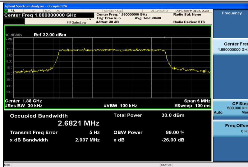
Band2-3MHz-16QAM-18900-15RB#0-2.6821
