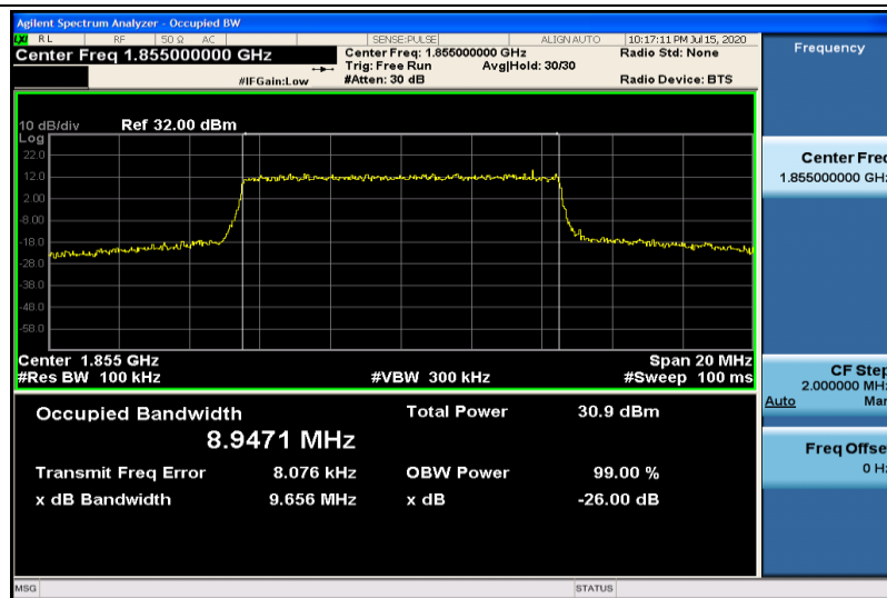
Band2-10MHz-16QAM-18650-50RB#0-8.9471
