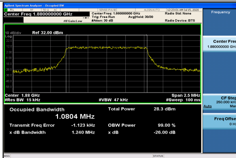
Band2-1.4MHz-QPSK-18900-6RB#0-1.0804
