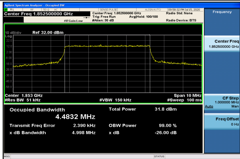
Band2-5MHz-QPSK-18625-25RB#0-4.4832
