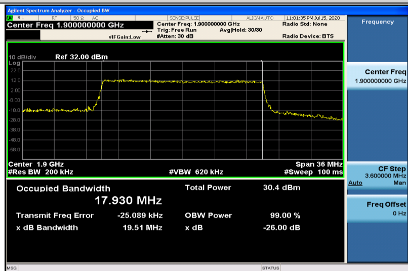
Band2-20MHz-16QAM-19100-100RB#0-17.930
