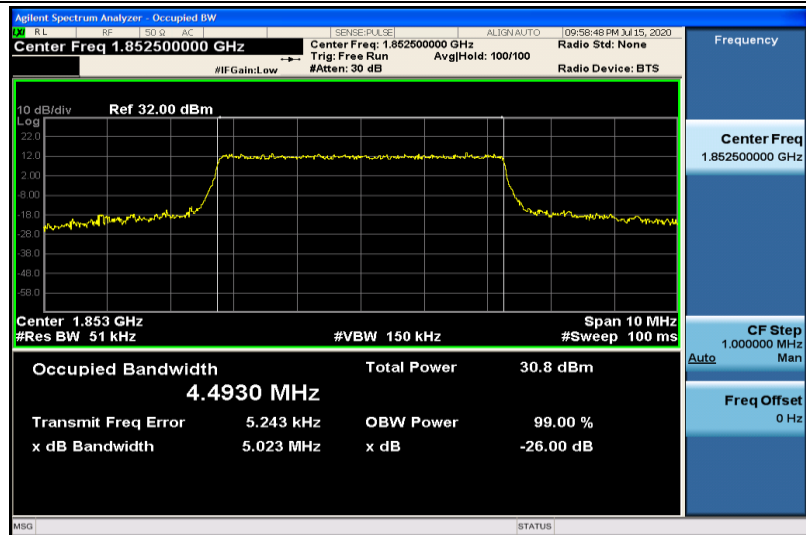
Band2-5MHz-16QAM-18625-25RB#0-4.4930
