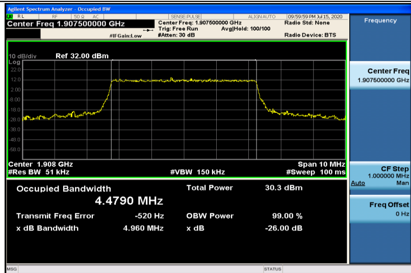
Band2-5MHz-16QAM-19175-25RB#0-4.4790
