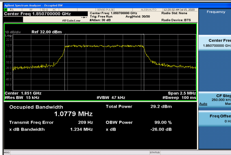
Band2-1.4MHz-QPSK-18607-6RB#0-1.0779
