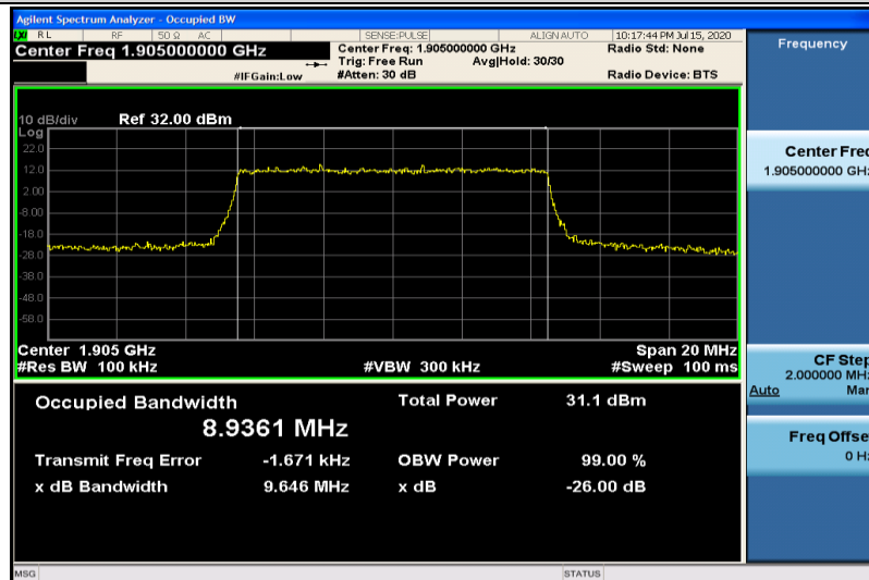
Band2-10MHz-QPSK-19150-50RB#0-8.9361
