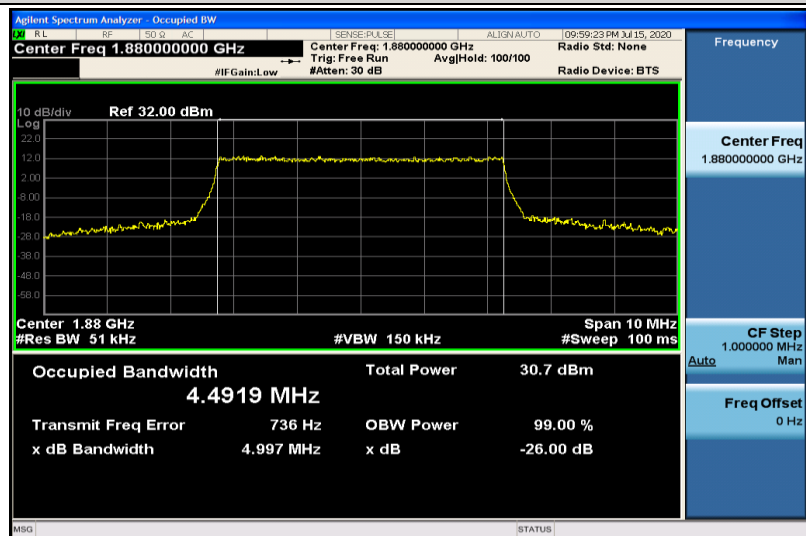
Band2-5MHz-16QAM-18900-25RB#0-4.4919
