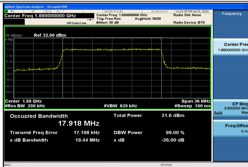
Band2-20MHz-QPSK-18900-100RB#0-17.918
