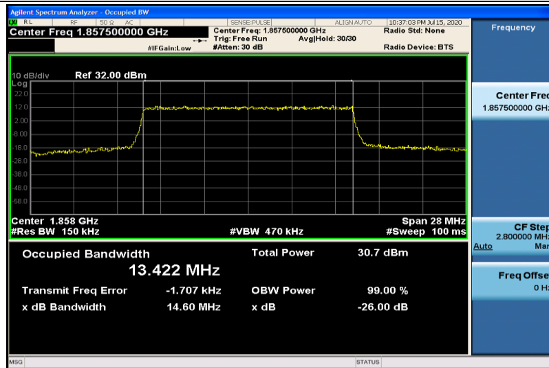
Band2-15MHz-16QAM-18675-75RB#0-13.422
