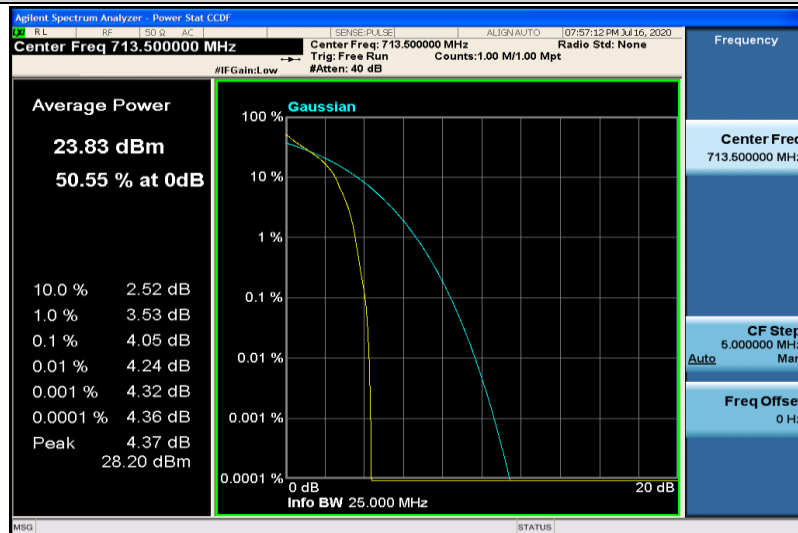
Band17-5MHz-QPSK-23825-1RB#0
