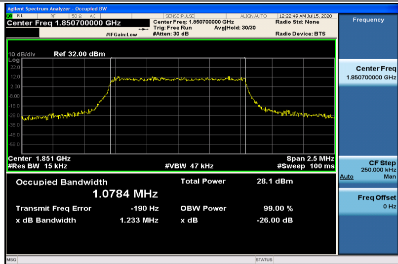
Band2-1.4MHz-16QAM-18607-6RB#0-1.0784
