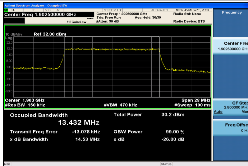
Band2-15MHz-16QAM-19125-75RB#0-13.432
