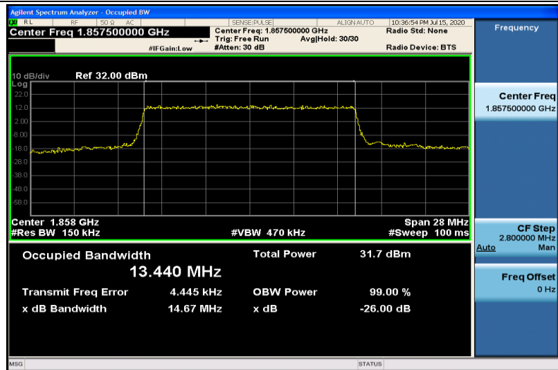
Band2-15MHz-QPSK-18675-75RB#0-13.440
