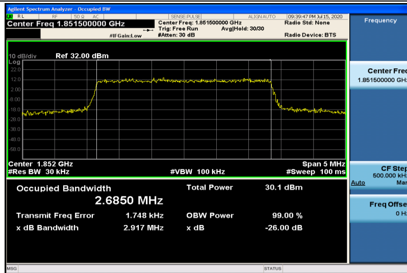
Band2-3MHz-16QAM-18615-15RB#0-2.6850
