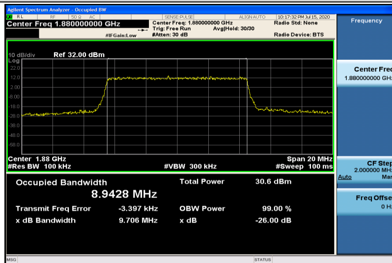
Band2-10MHz-16QAM-18900-50RB#0-8.9428
