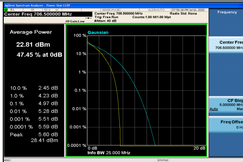
Band17-5MHz-QPSK-23755-25RB#0
