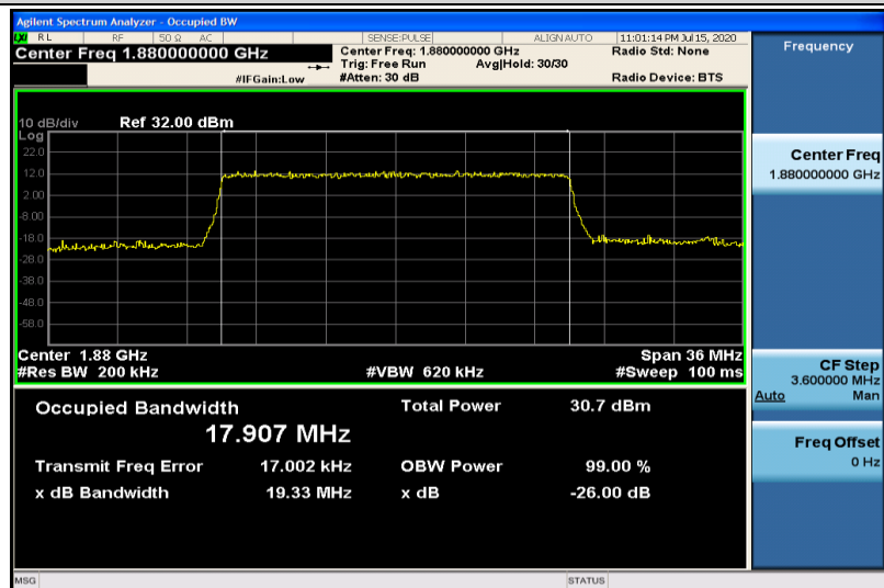
Band2-20MHz-16QAM-18900-100RB#0-17.907
