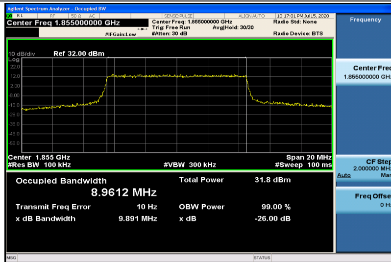
Band2-10MHz-QPSK-18650-50RB#0-8.9612
