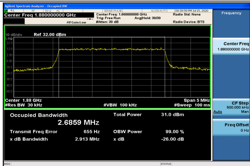
Band2-3MHz-QPSK-18900-15RB#0-2.6859
