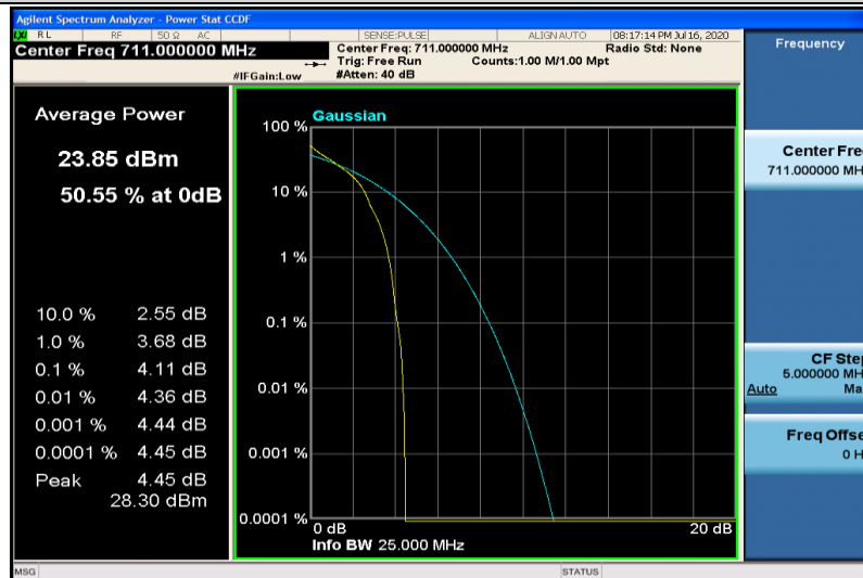
Band17-10MHz-QPSK-23800-1RB#0
