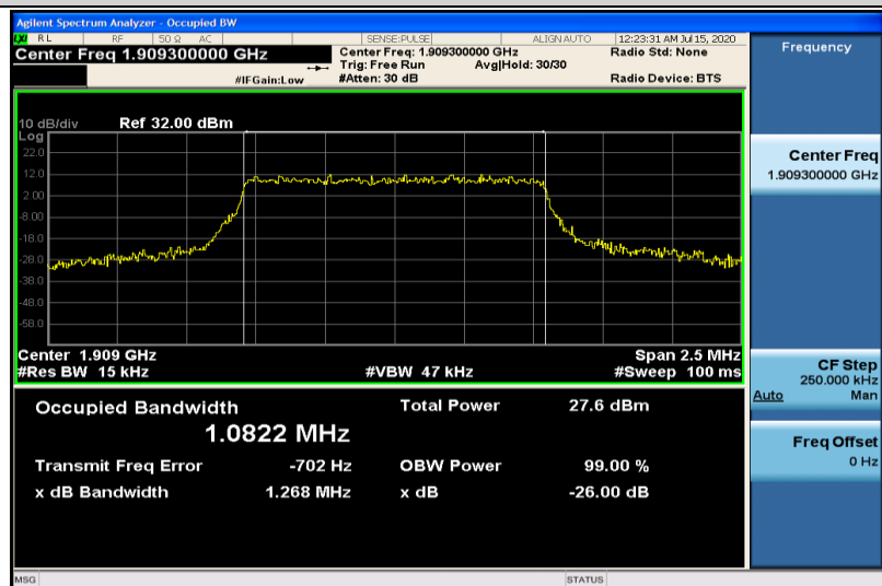
Band2-1.4MHz-16QAM-19193-6RB#0-1.0822
