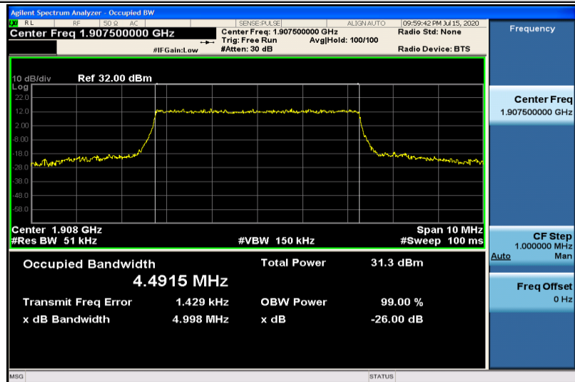
Band2-5MHz-QPSK-19175-25RB#0-4.4915
