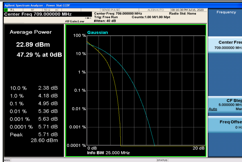
Band17-10MHz-QPSK-23780-50RB#0
