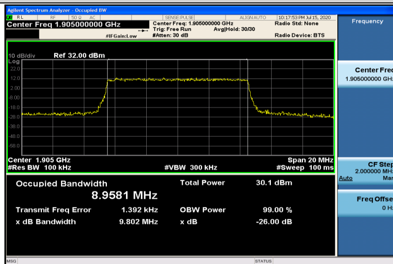
Band2-10MHz-16QAM-19150-50RB#0-8.9581
