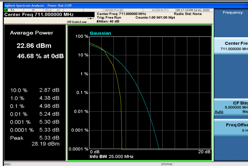
Band17-10MHz-16QAM-23800-1RB#0
