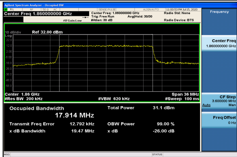
Band2-20MHz-16QAM-18700-100RB#0-17.914
