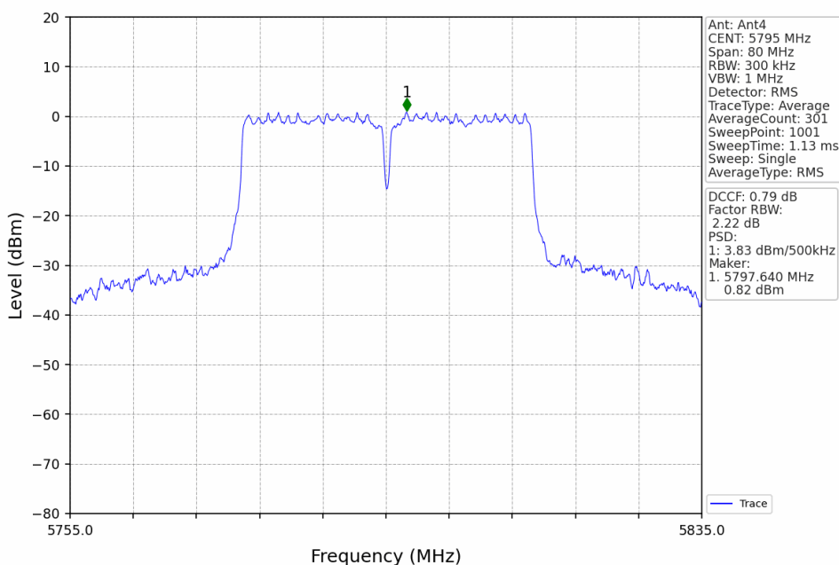
802.11ac(VHT40)_HCH_5795MHz_Ant4_NTNV
