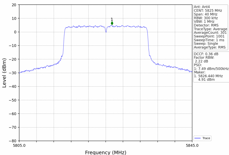
802.11ax(HEW20)_HCH_5825MHz_RU242_Left_Ant4_NTNV
