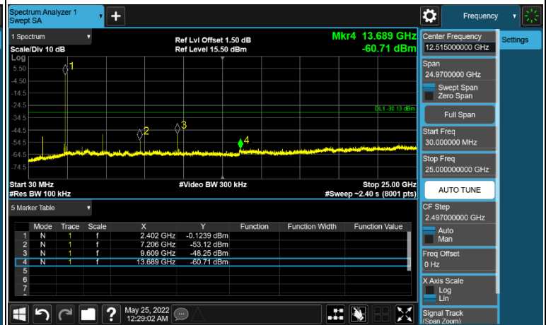
Mode 1 CH00(2402MHz)
