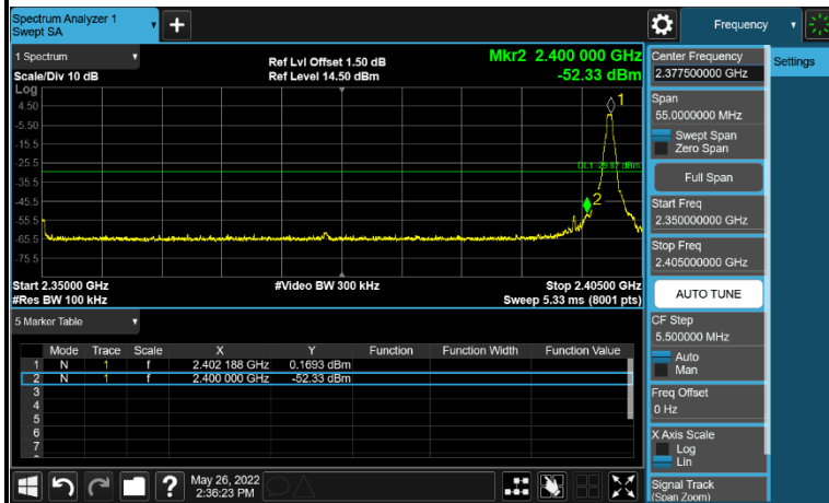
Mode 1 CH00(2402MHz)
