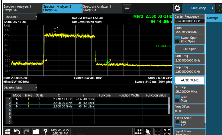
Mode 6 (3DH5- Hopping)
