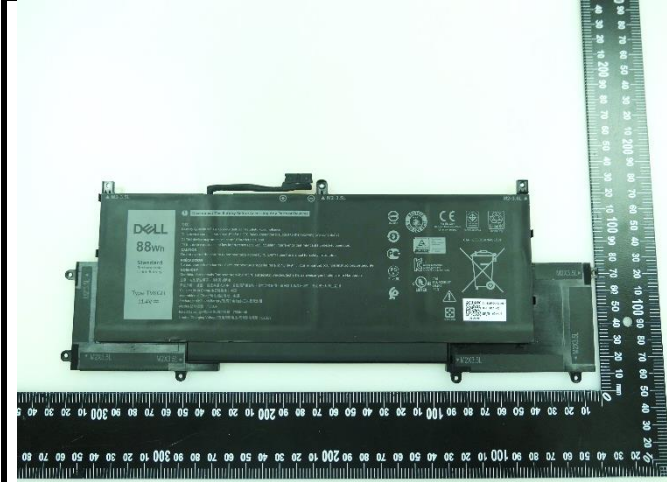
Battery (6 Cell)
