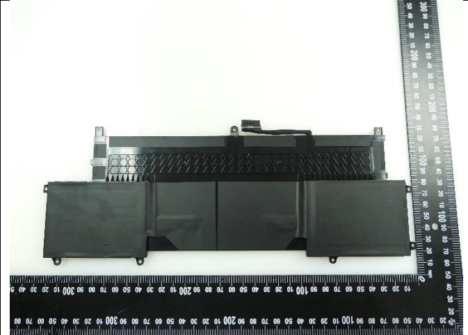
Battery (6 Cell)
