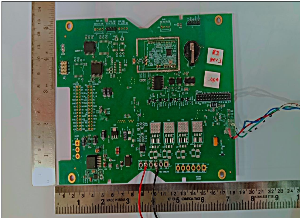
Figure 3: PCB Dimensional view
