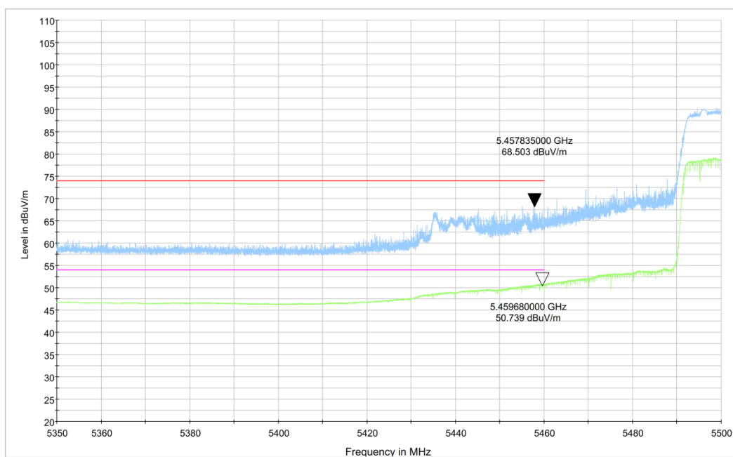
Fig.56 Band Edges (802.11ac-HT80 Ch106, 5530MHz)
