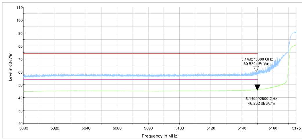
Fig.38 Band Edges (802.11n-HT20 Ch36, 5180MHz)
