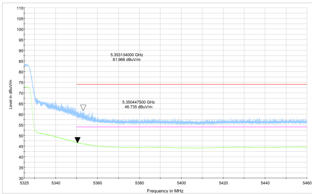
Fig.51 Band Edges (802.11ac-HT40 Ch62, 5310MHz)
