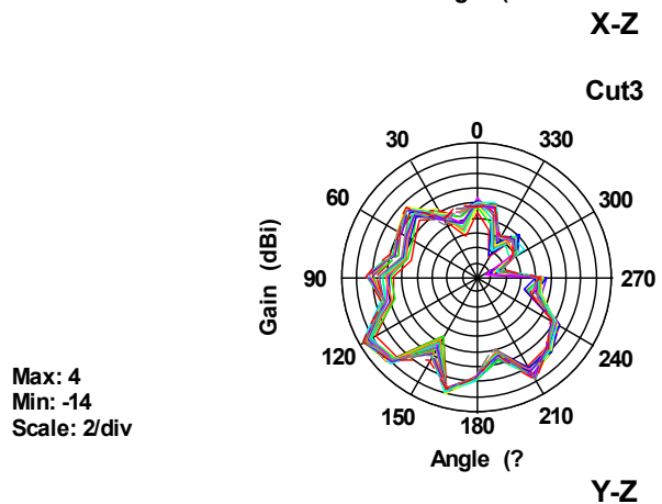
2397MHz- 2497 MHz Wi-Fi 2.4G 3D Gain
