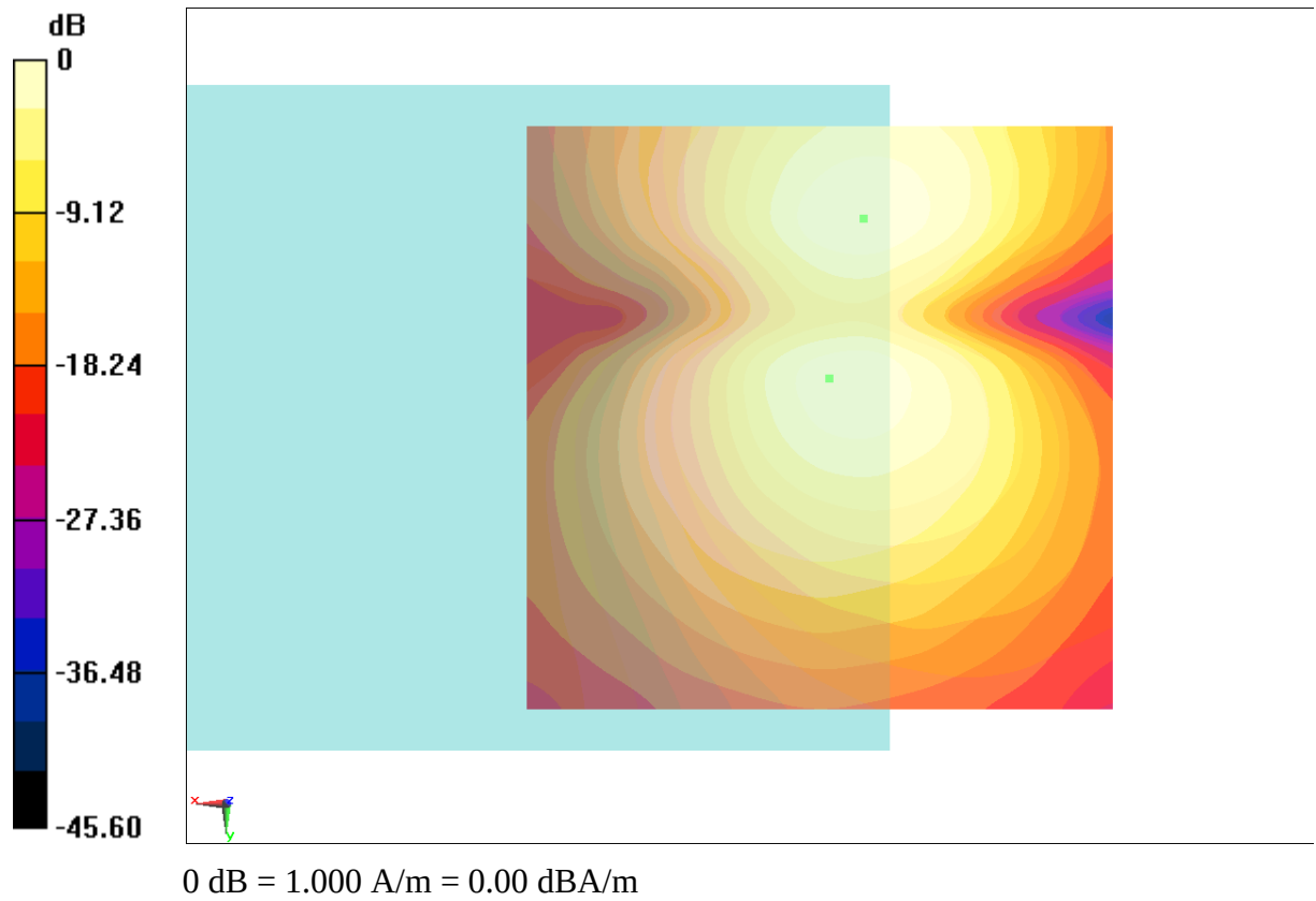
Fig B.6 T-Coil GSM 1900
