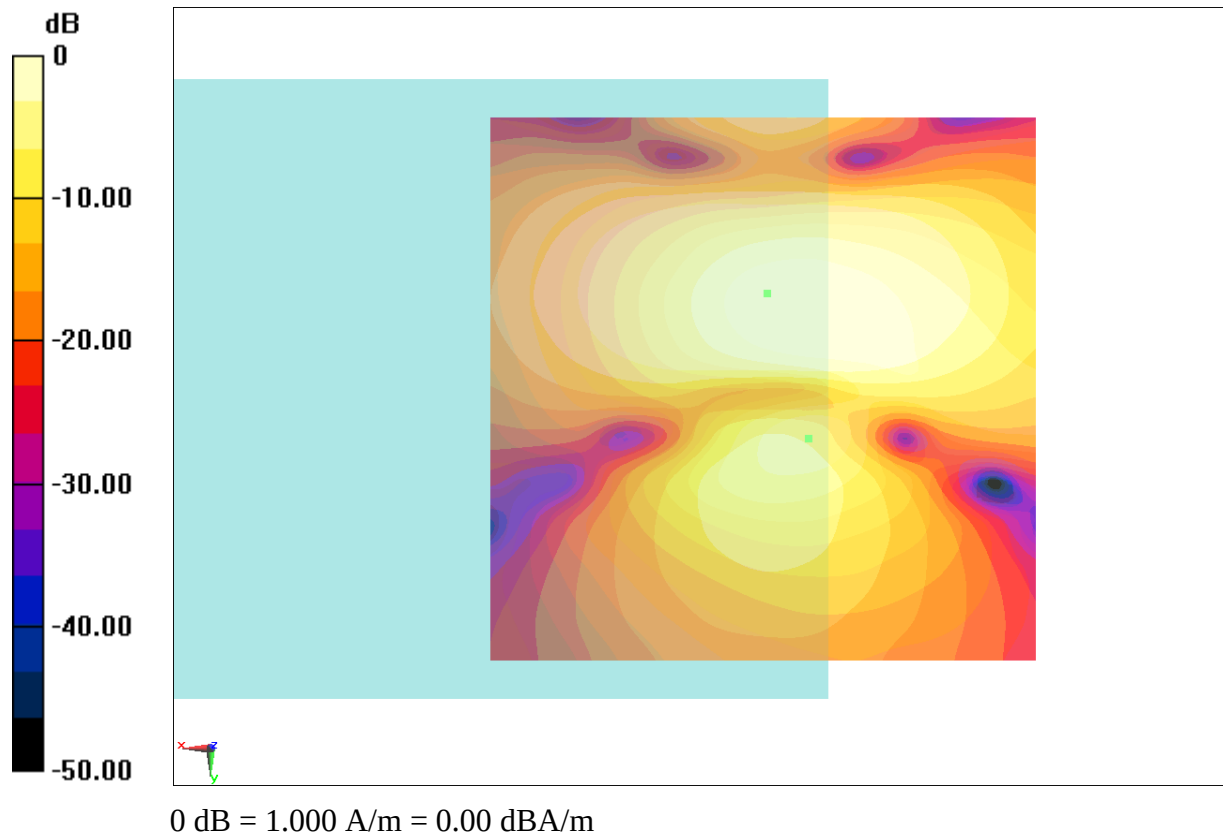
Fig B.5 T-Coil GSM 1900
