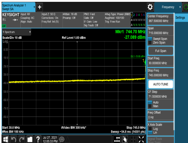
Plot 7-445. Conducted Spurious Emission Plot 30 MHz to 745 MHz (Multi Band_B5_5M_1C_Low + B13_5M_1C_High_QPSK - Port 3)
