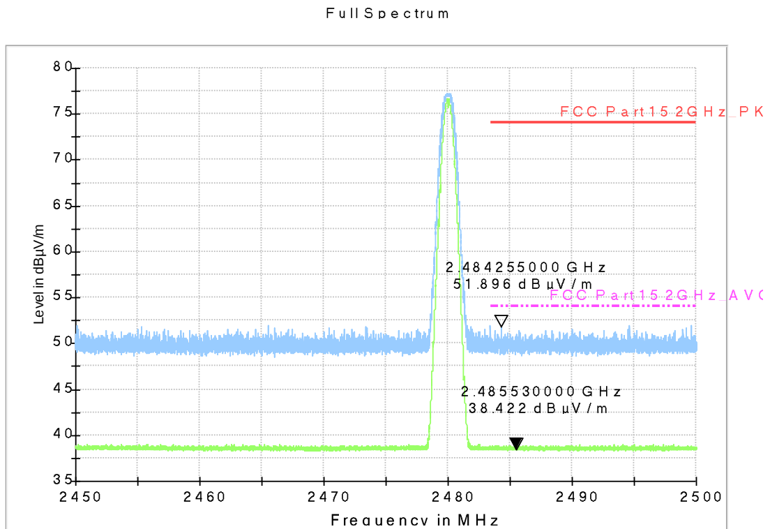
Fig.59. Radiated emission (Power) GFSK, high channel
