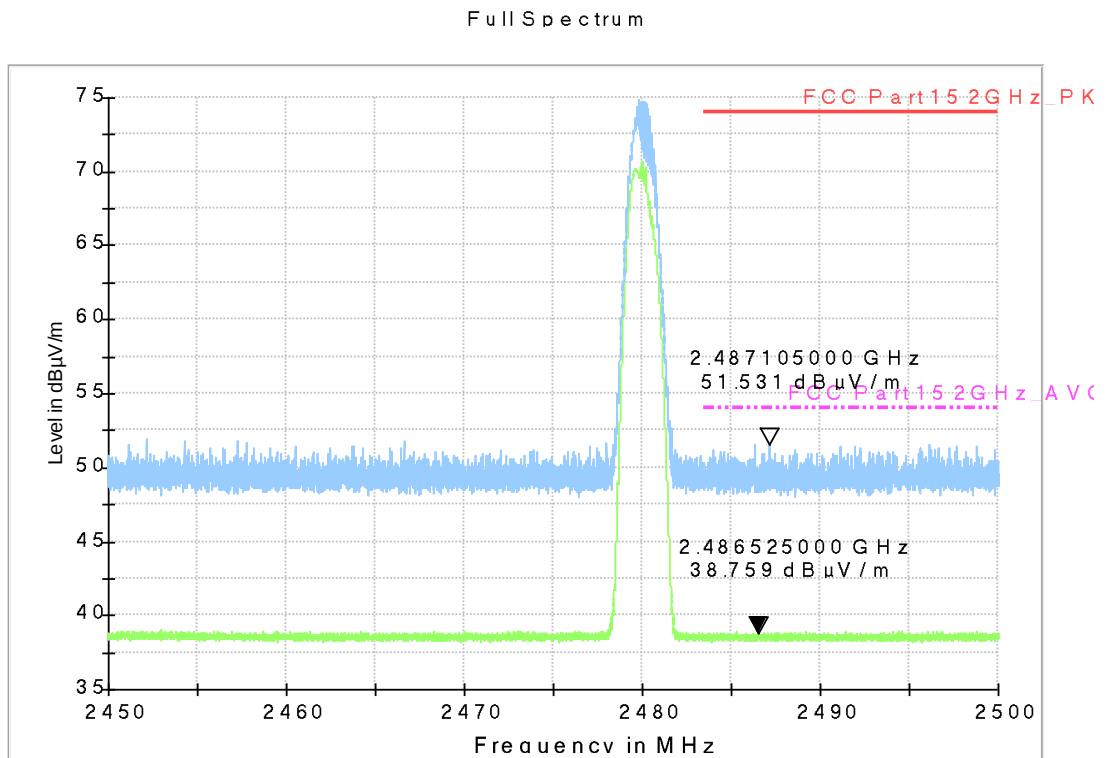
Fig.63. Radiated emission (Power): 8DPSK, high channel
