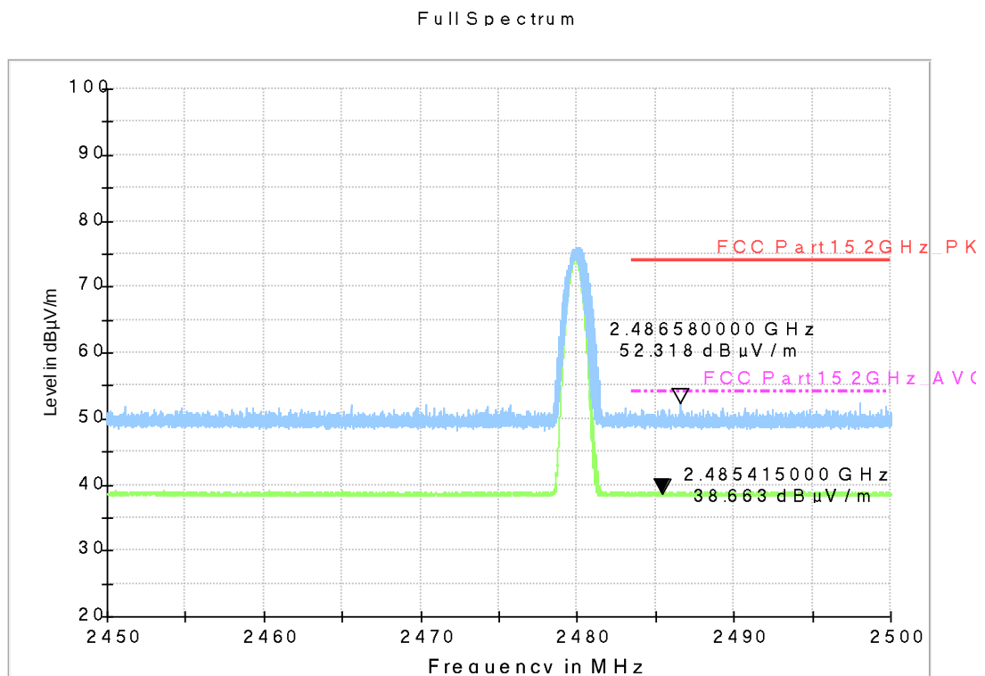
Fig.61. Radiated emission (Power): \pi/4 DQPSK, high channel
