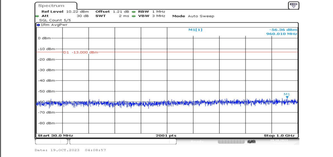
Band25-10MHz-QPSK-26640-1RB#0-Range3:30~1000MHz-PASS
