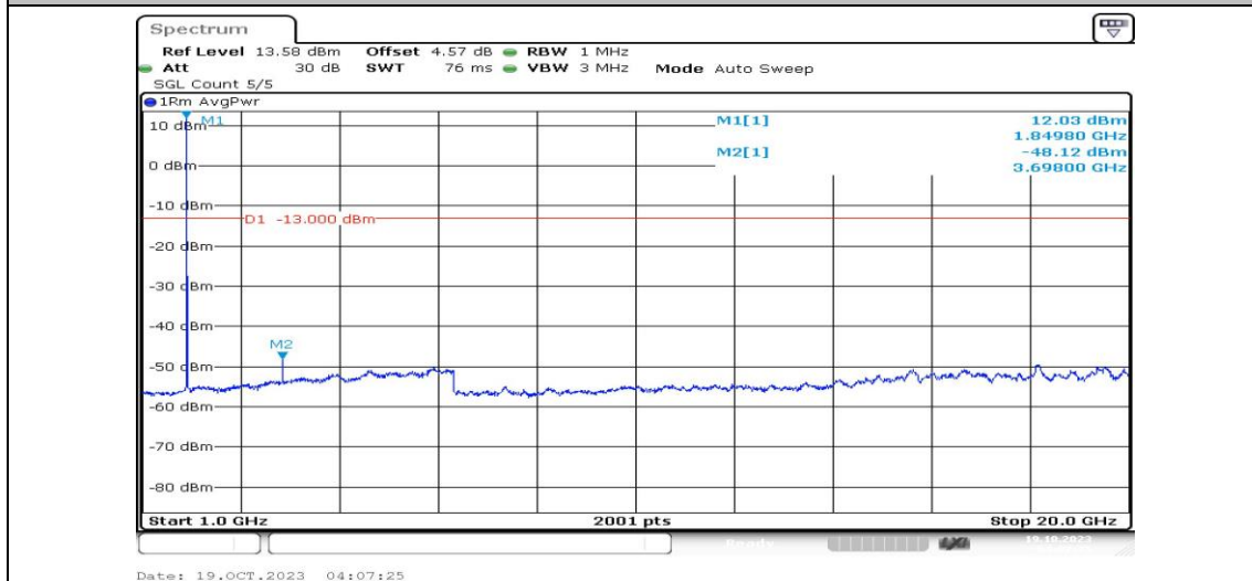
Band25-10MHz-QPSK-26090-1RB#0-Range4:1000~20000MHz-PASS
