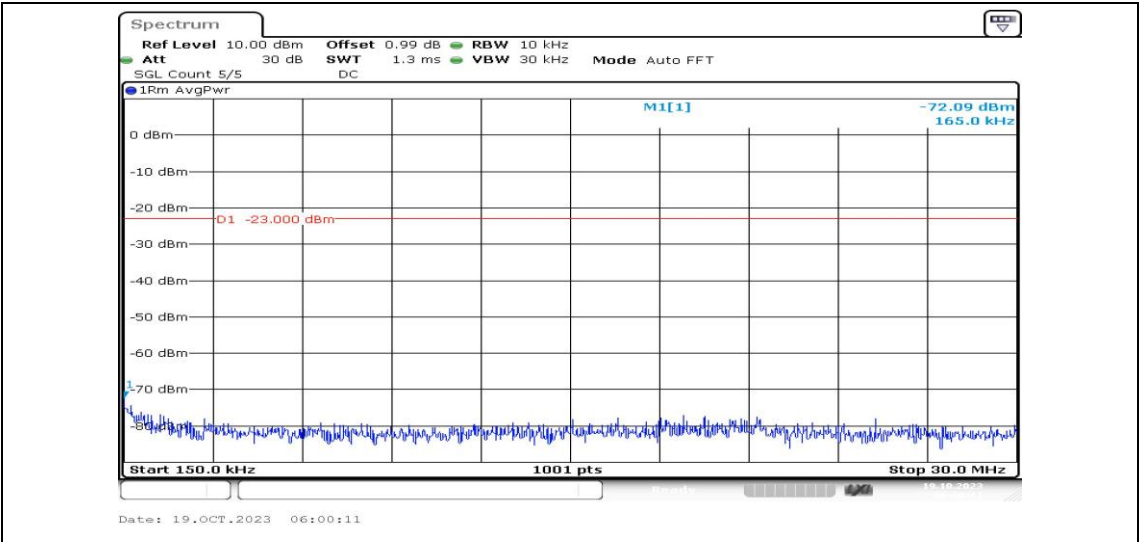
Band25-15MHz-16QAM-26365-1RB#0-Range2:0.15~30MHz-PASS
