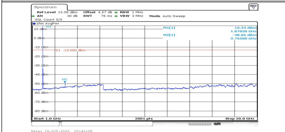
Band25-10MHz-16QAM-26365-1RB#0-Range4:1000~20000MHz-PASS
