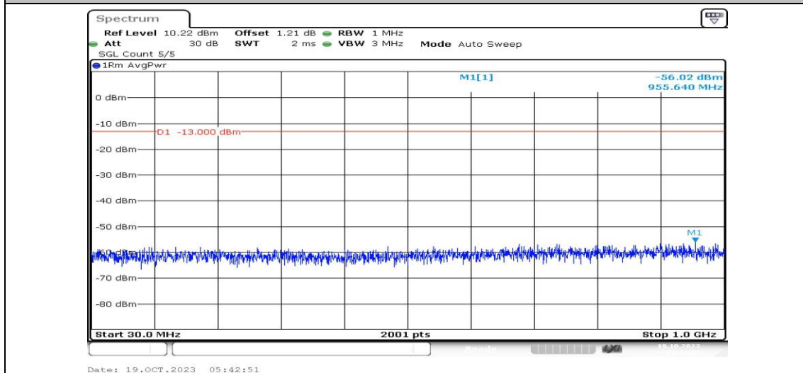
Band25-10MHz-16QAM-26365-1RB#0-Range3:30~1000MHz-PASS
