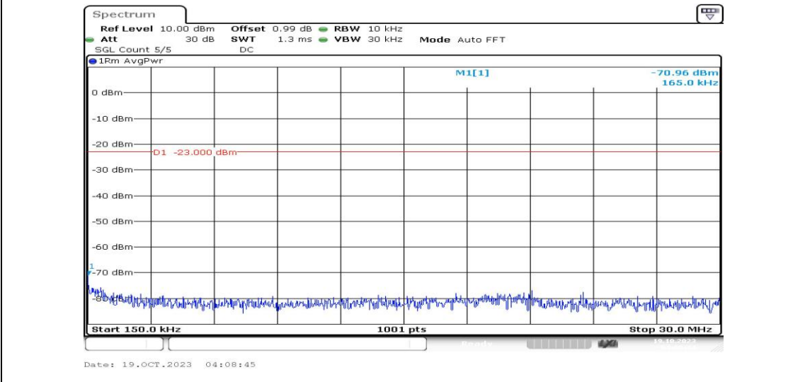
Band25-10MHz-QPSK-26640-1RB#0-Range2:0.15~30MHz-PASS
