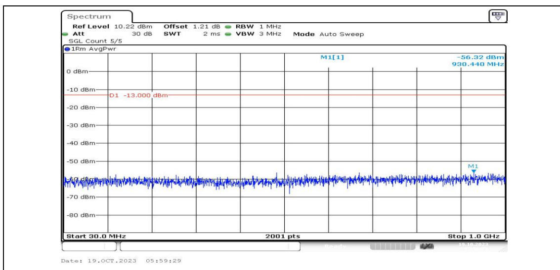
Band25-15MHz-16QAM-26115-1RB#0-Range3:30~1000MHz-PASS
