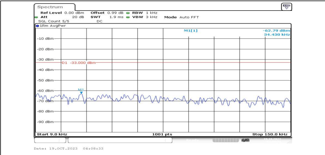
Band25-10MHz-QPSK-26640-1RB#0-Range1:0.009~0.15MHz-PASS
