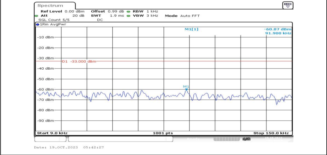
Band25-10MHz-16QAM-26365-1RB#0-Range1:0.009~0.15MHz-PASS
