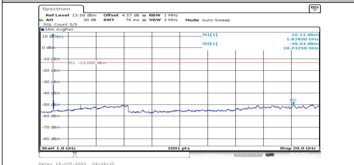
Band25-15MHz-QPSK-26365-1RB#0-Range4:1000~20000MHz-PASS
