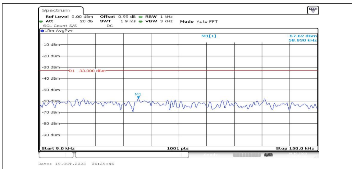
Band25-20MHz-16QAM-26590-1RB#0-Range1:0.009~0.15MHz-PASS
