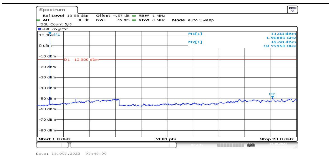
Band25-10MHz-16QAM-26640-1RB#0-Range4:1000~20000MHz-PASS
