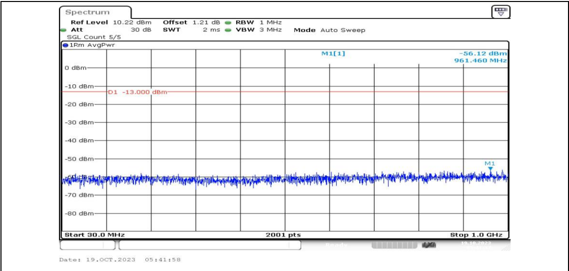
Band25-10MHz-16QAM-26090-1RB#0-Range3:30~1000MHz-PASS
