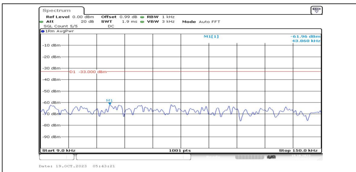
Band25-10MHz-16QAM-26640-1RB#0-Range1:0.009~0.15MHz-PASS
