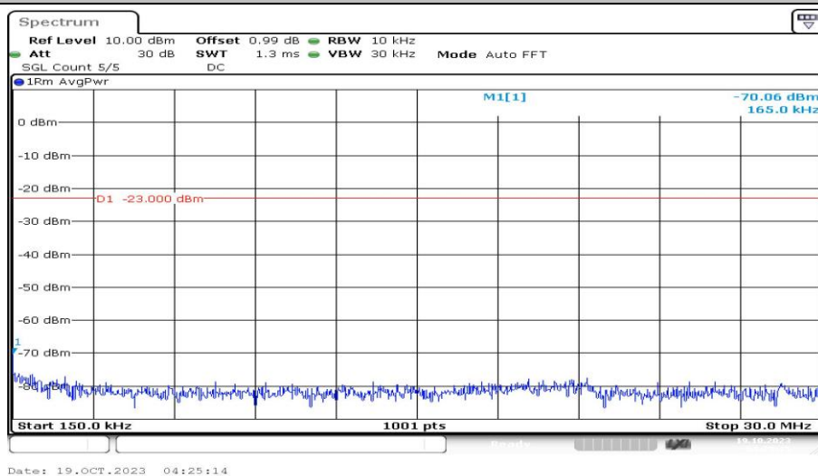
Band25-15MHz-QPSK-26115-1RB#0-Range2:0.15~30MHz-PASS
