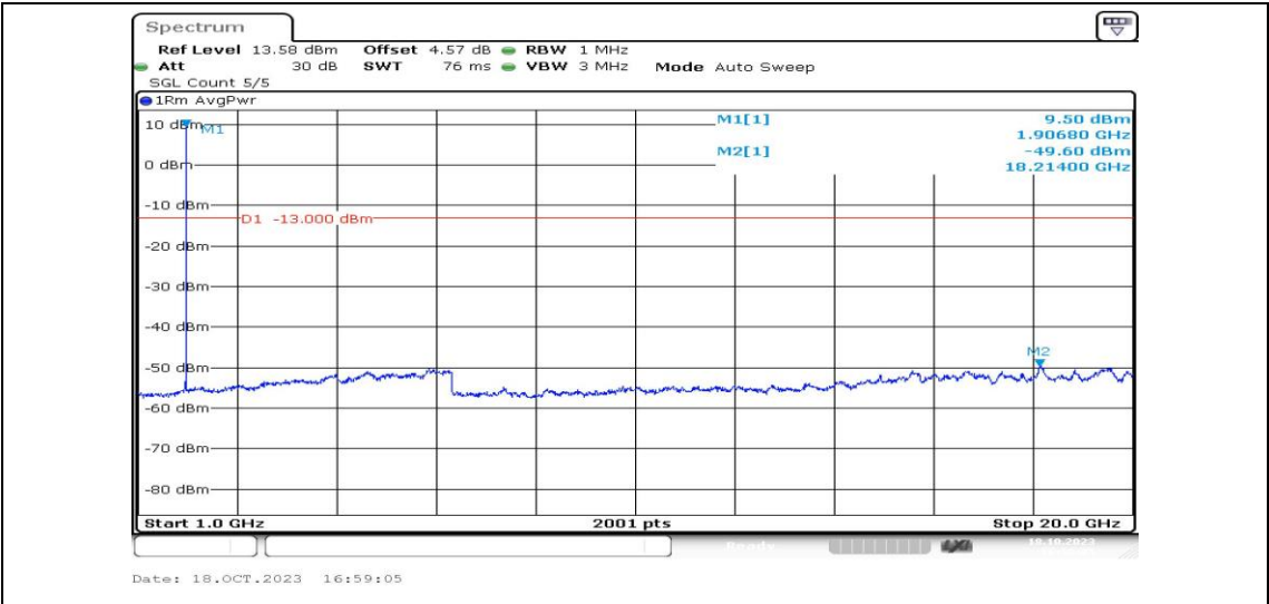
Band25-5MHz-16QAM-26665-1RB#0-Range4:1000~20000MHz-PASS
