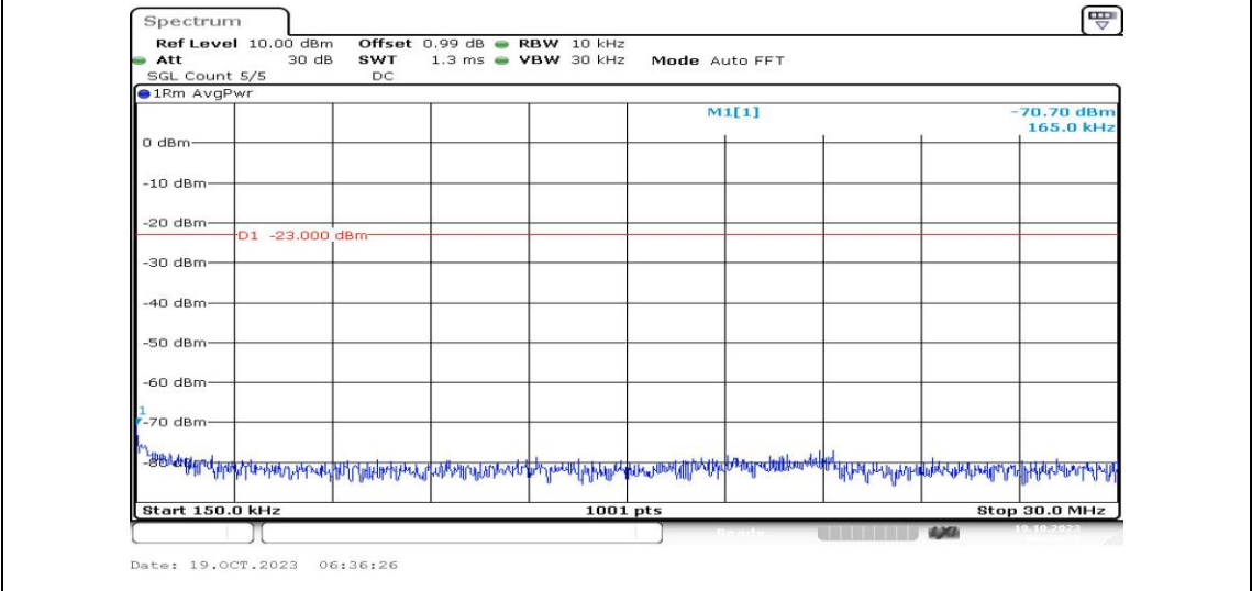
Band25-20MHz-16QAM-26140-1RB#0-Range2:0.15~30MHz-PASS
