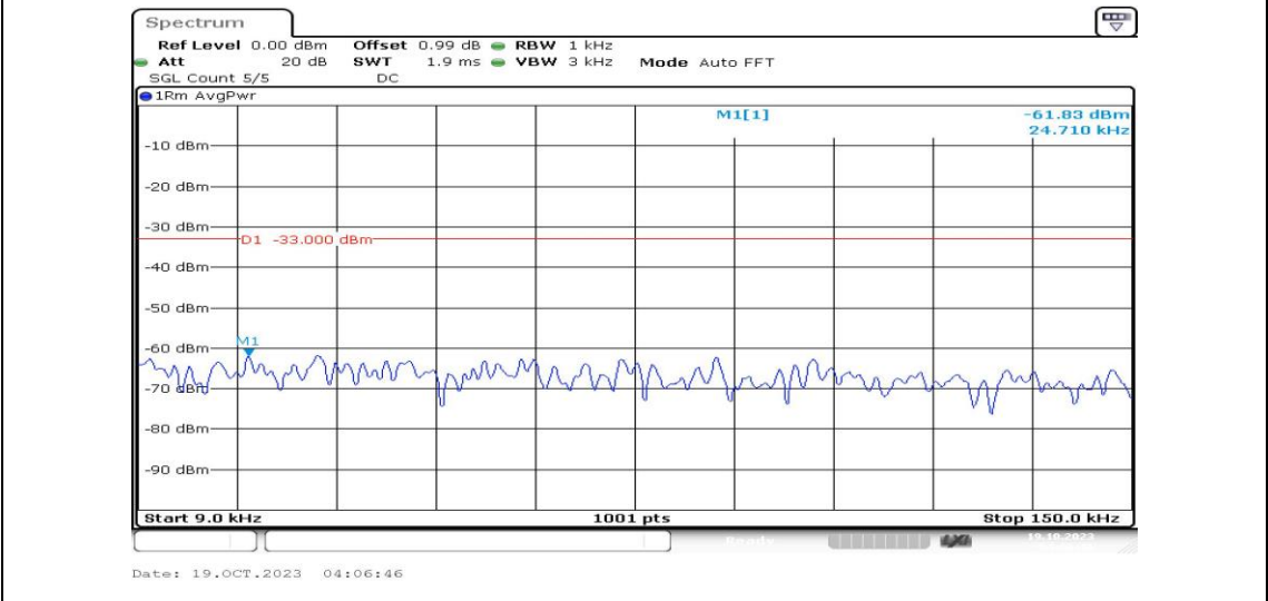
Band25-10MHz-QPSK-26090-1RB#0-Range1:0.009~0.15MHz-PASS
