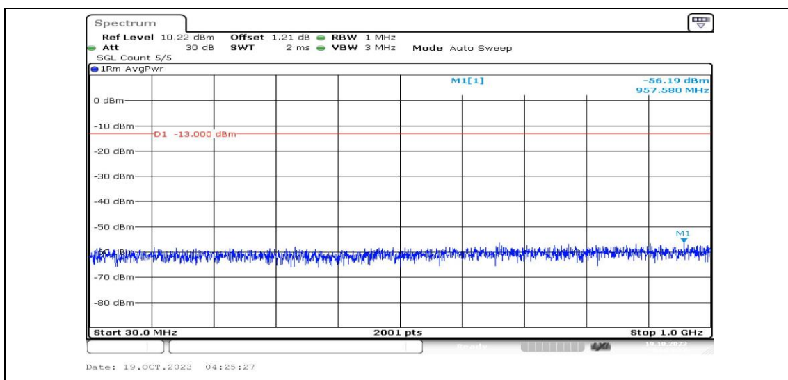
Band25-15MHz-QPSK-26115-1RB#0-Range3:30~1000MHz-PASS
