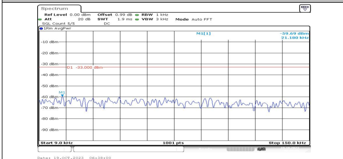
Band25-20MHz-16QAM-26365-1RB#0-Range1:0.009~0.15MHz-PASS
