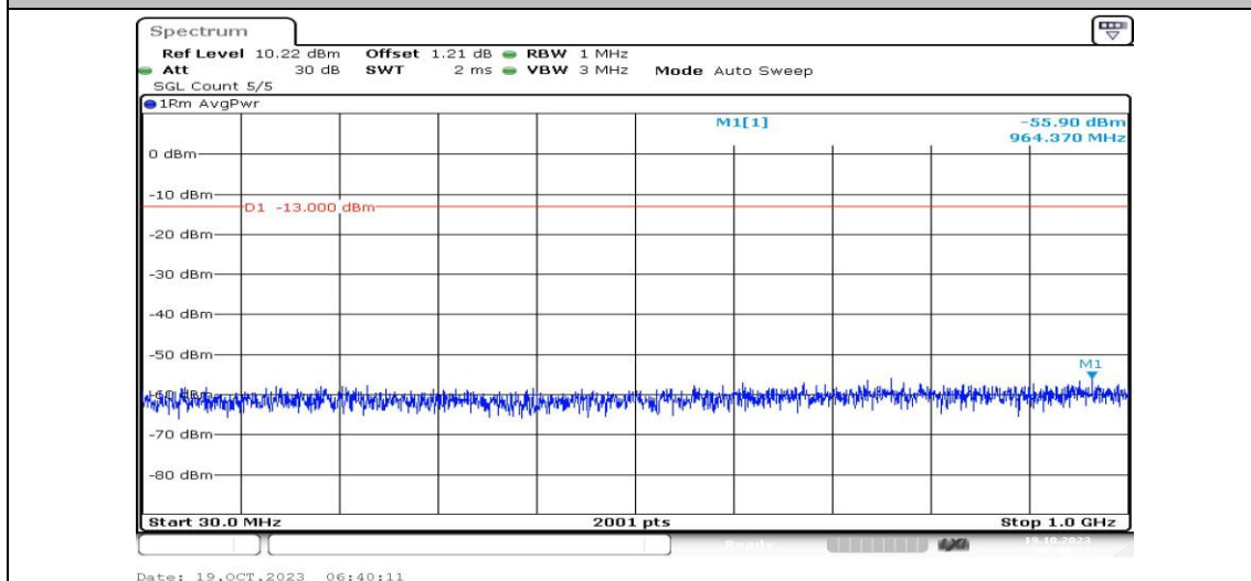
Band25-20MHz-16QAM-26590-1RB#0-Range3:30~1000MHz-PASS
