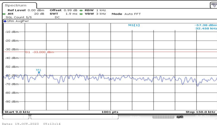
Band25-20MHz-QPSK-26140-1RB#0-Range1:0.009~0.15MHz-PASS
