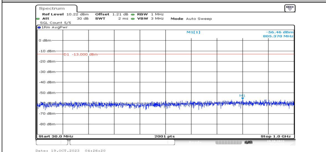
Band25-15MHz-QPSK-26365-1RB#0-Range3:30~1000MHz-PASS
