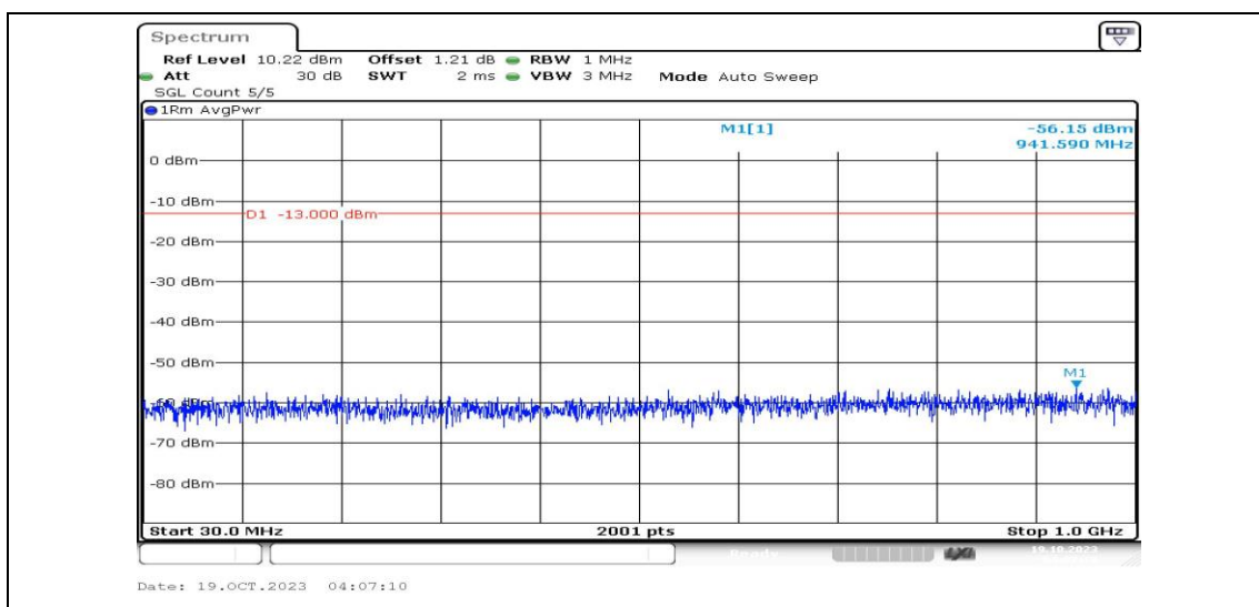
Band25-10MHz-QPSK-26090-1RB#0-Range3:30~1000MHz-PASS
