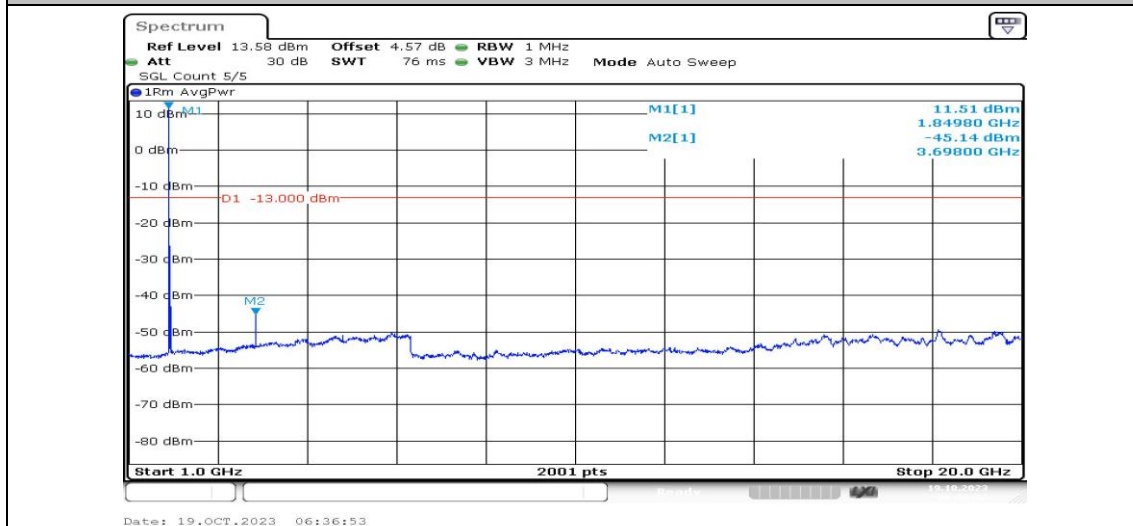
Band25-20MHz-16QAM-26140-1RB#0-Range4:1000~20000MHz-PASS
