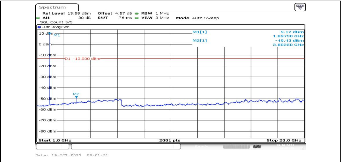
Band25-15MHz-16QAM-26615-1RB#0-Range4:1000~20000MHz-PASS
