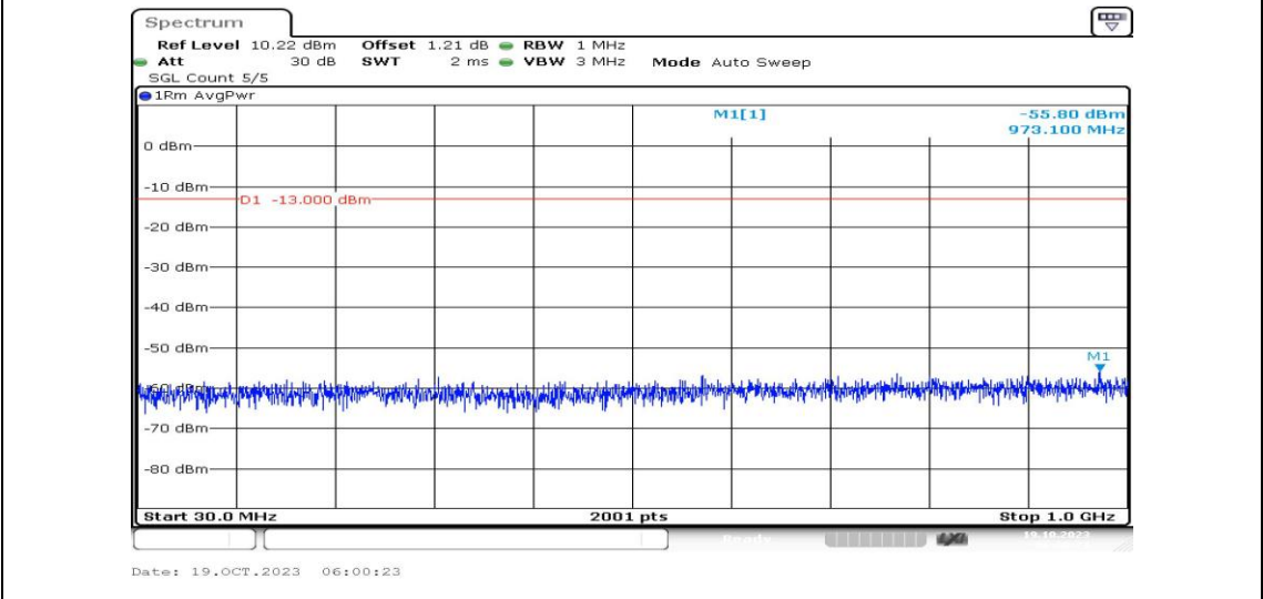
Band25-15MHz-16QAM-26365-1RB#0-Range3:30~1000MHz-PASS
