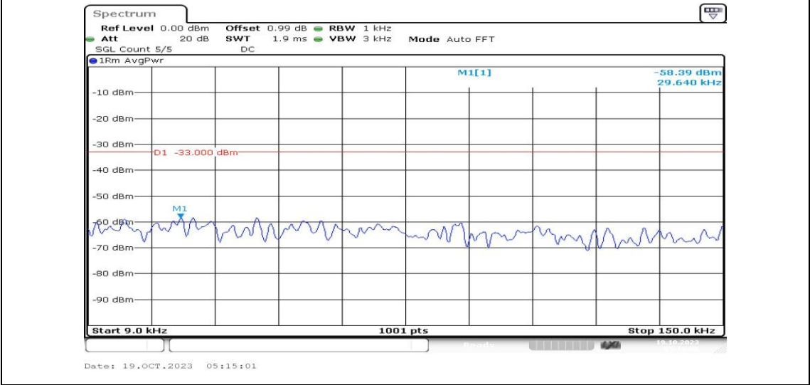
Band25-20MHz-QPSK-26365-1RB#0-Range1:0.009~0.15MHz-PASS
