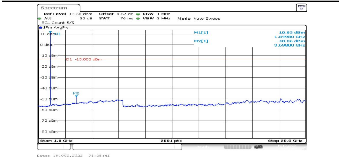
Band25-15MHz-QPSK-26115-1RB#0-Range4:1000~20000MHz-PASS
