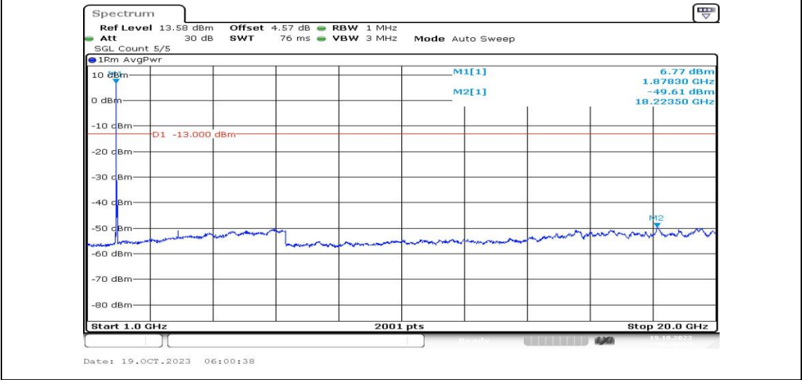
Band25-15MHz-16QAM-26365-1RB#0-Range4:1000~20000MHz-PASS
