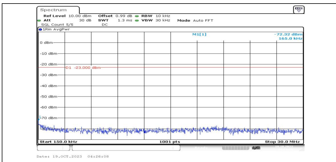
Band25-15MHz-QPSK-26365-1RB#0-Range2:0.15~30MHz-PASS
