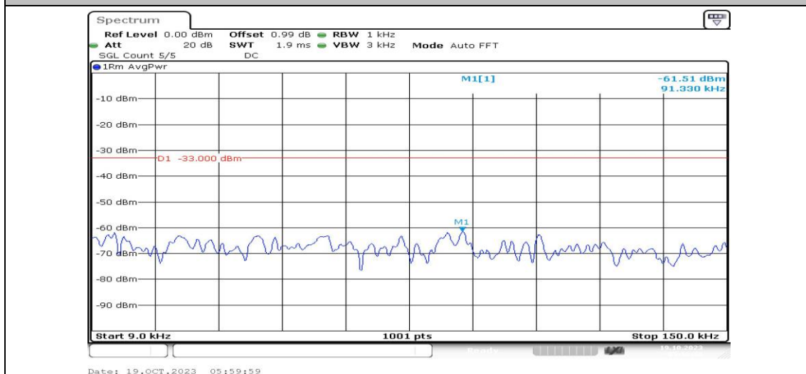
Band25-15MHz-16QAM-26365-1RB#0-Range1:0.009~0.15MHz-PASS
