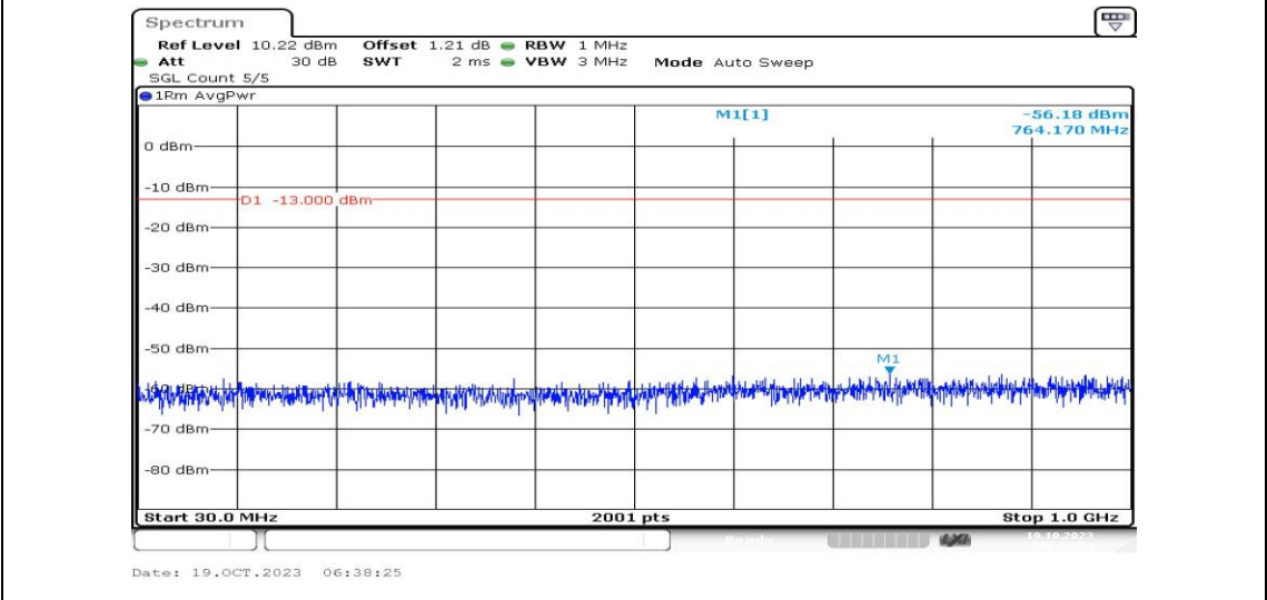
Band25-20MHz-16QAM-26365-1RB#0-Range3:30~1000MHz-PASS
