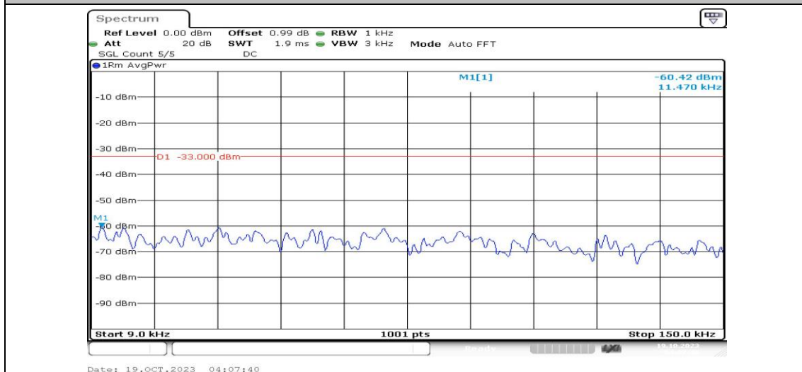
Band25-10MHz-QPSK-26365-1RB#0-Range1:0.009~0.15MHz-PASS
