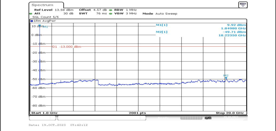
Band25-10MHz-16QAM-26090-1RB#0-Range4:1000~20000MHz-PASS
