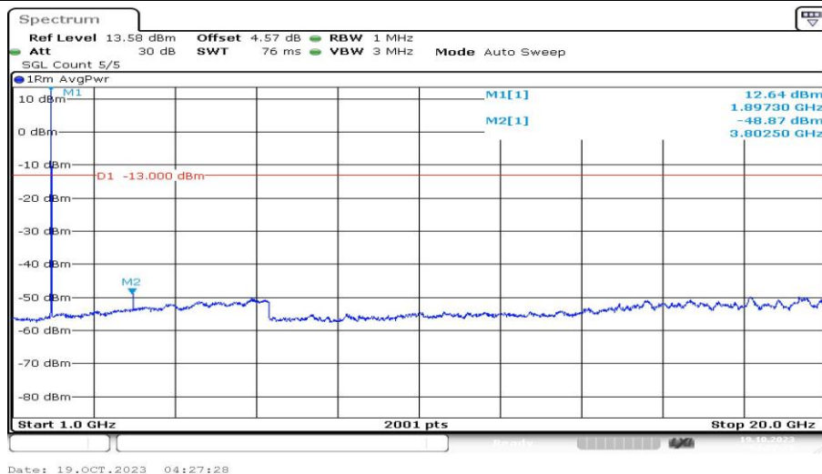
Band25-15MHz-QPSK-26615-1RB#0-Range4:1000~20000MHz-PASS
