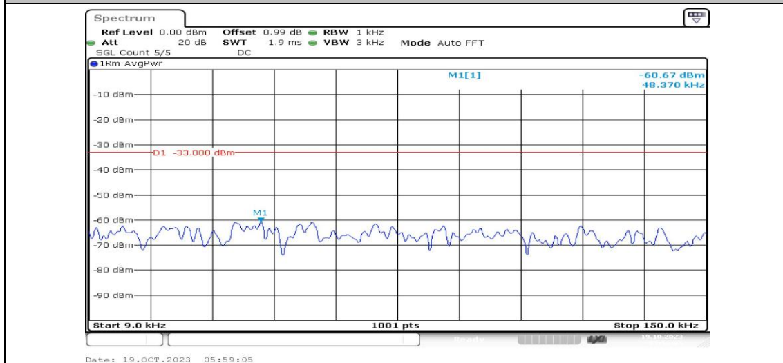
Band25-15MHz-16QAM-26115-1RB#0-Range1:0.009~0.15MHz-PASS
