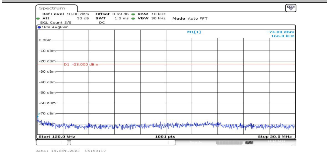
Band25-15MHz-16QAM-26115-1RB#0-Range2:0.15~30MHz-PASS
