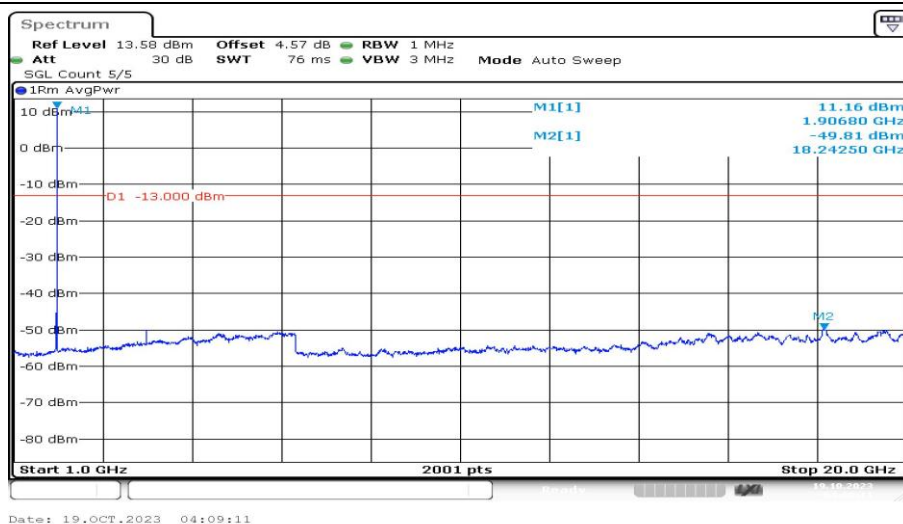
Band25-10MHz-QPSK-26640-1RB#0-Range4:1000~20000MHz-PASS
