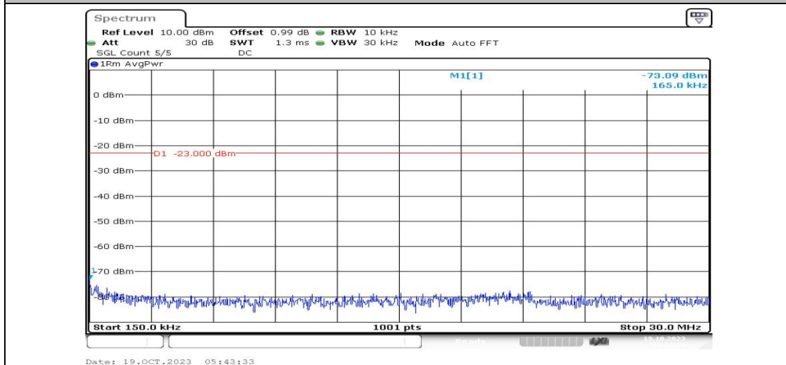
Band25-10MHz-16QAM-26640-1RB#0-Range2:0.15~30MHz-PASS
