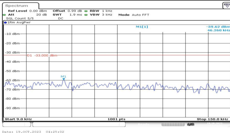
Band25-15MHz-QPSK-26115-1RB#0-Range1:0.009~0.15MHz-PASS
