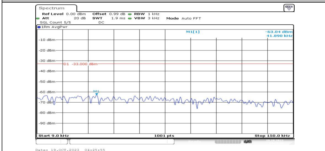
Band25-15MHz-QPSK-26365-1RB#0-Range1:0.009~0.15MHz-PASS
