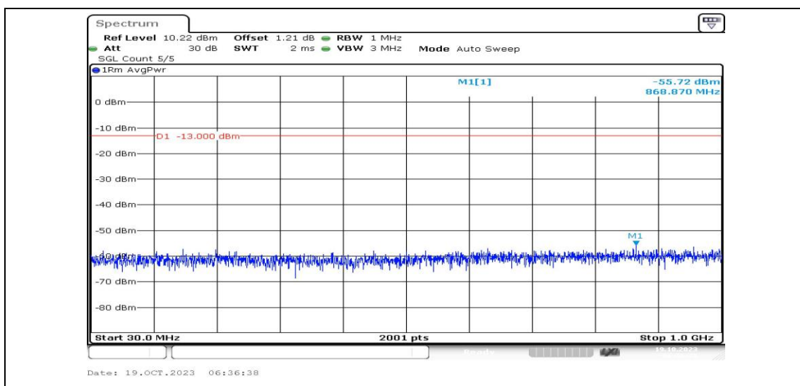
Band25-20MHz-16QAM-26140-1RB#0-Range3:30~1000MHz-PASS
